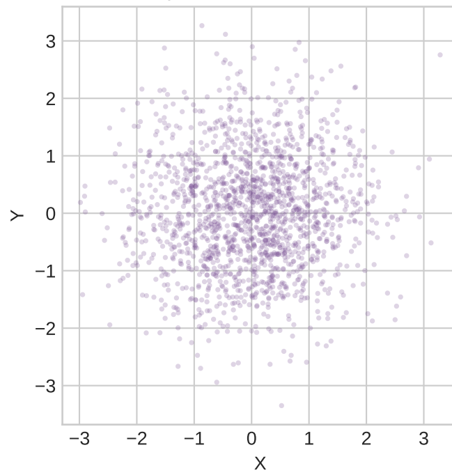
Two-driver planar Brownian law: rank two
