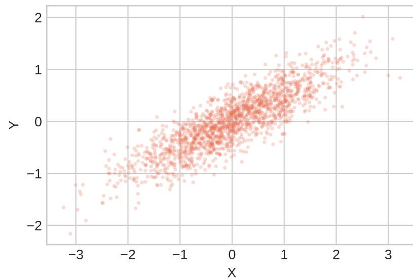
One driver, dY = Xdt : terminal rank two
