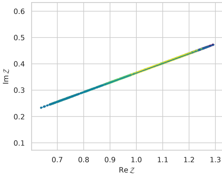
stochastic rotation: \omega = 0.0 , \beta = 1.0
