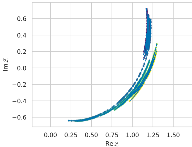
stochastic rotation: \omega = 0.0 , \beta = 1.0
