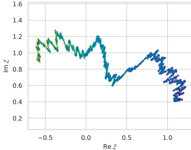
combined rotation: \omega = 1.2 , \beta = 1.0
