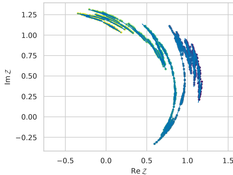
combined rotation: \omega = 1.2 , \beta = 1.0
