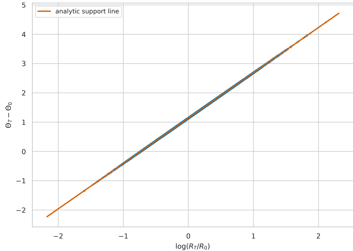
Fixed-horizon transition law in log-polar coordinates
