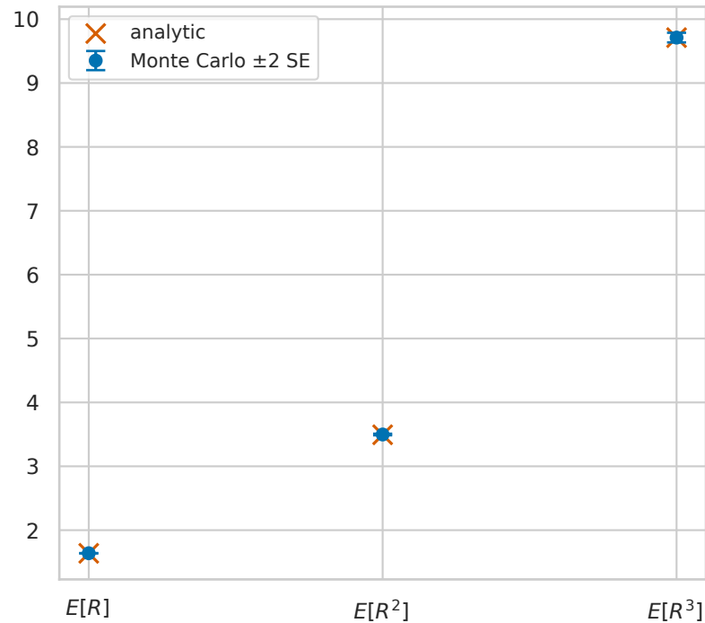
Radial moments
