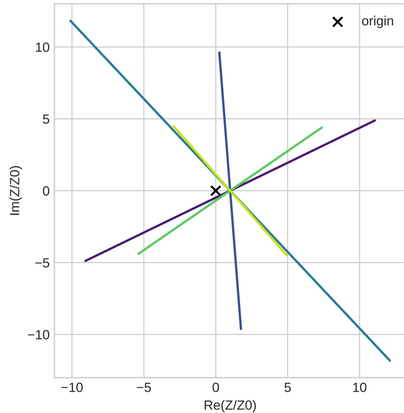
Eligible normalized support lines miss the origin
