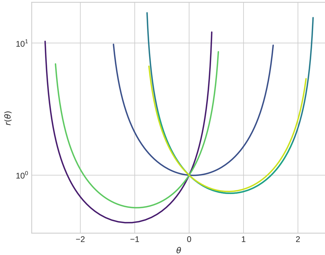
Each positive polar branch spans exactly one half-turn
