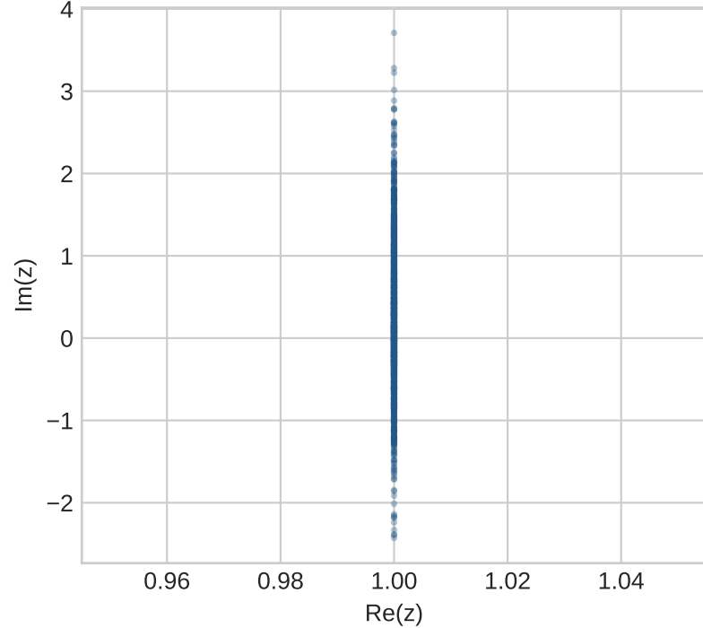
Collinear: rank-one fixed line
