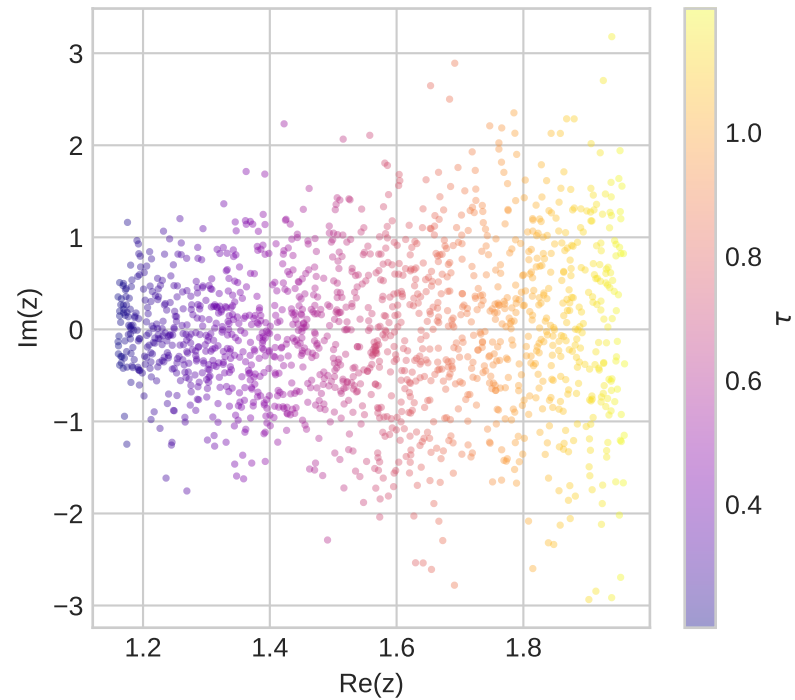
Noncollinear + random time: planar density
