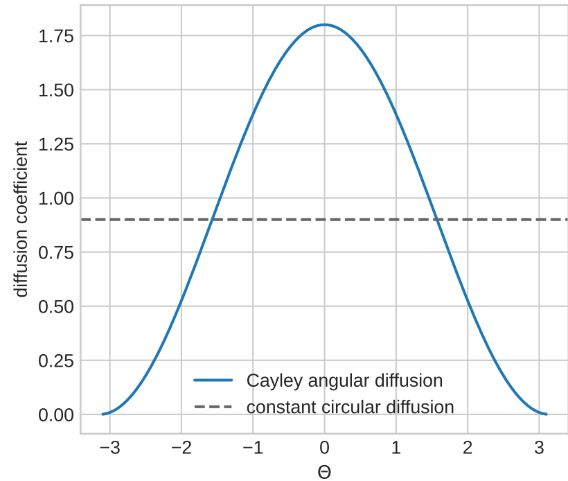
Not ordinary Brownian motion on a circle
