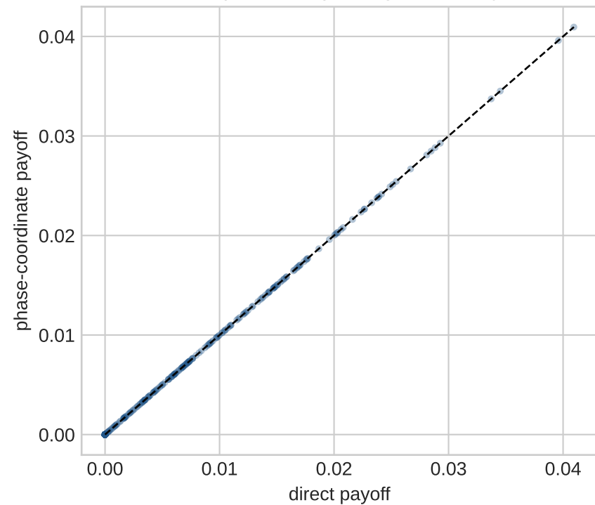
European samples agree exactly
