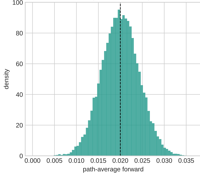
Common terminal phase, different path averages
