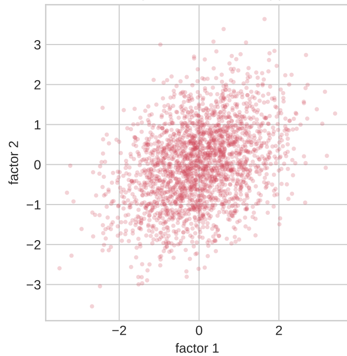
Nonsingular two-factor support
