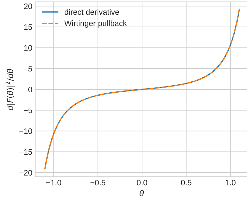
Wirtinger calculus repackages two real derivatives
