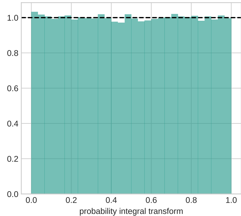
PIT: KS=0.0024
