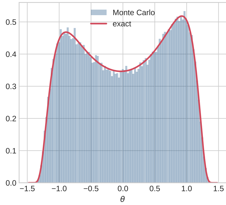
Transformed-normal density
