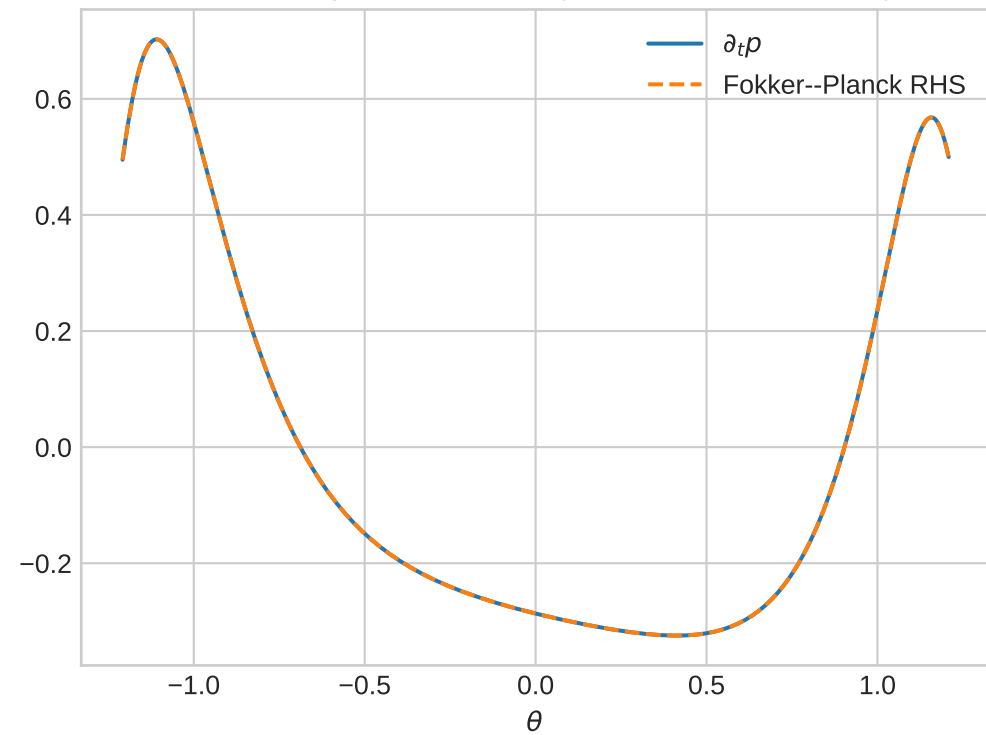
Forward equation residual (relative RMS 6.90e-05)
