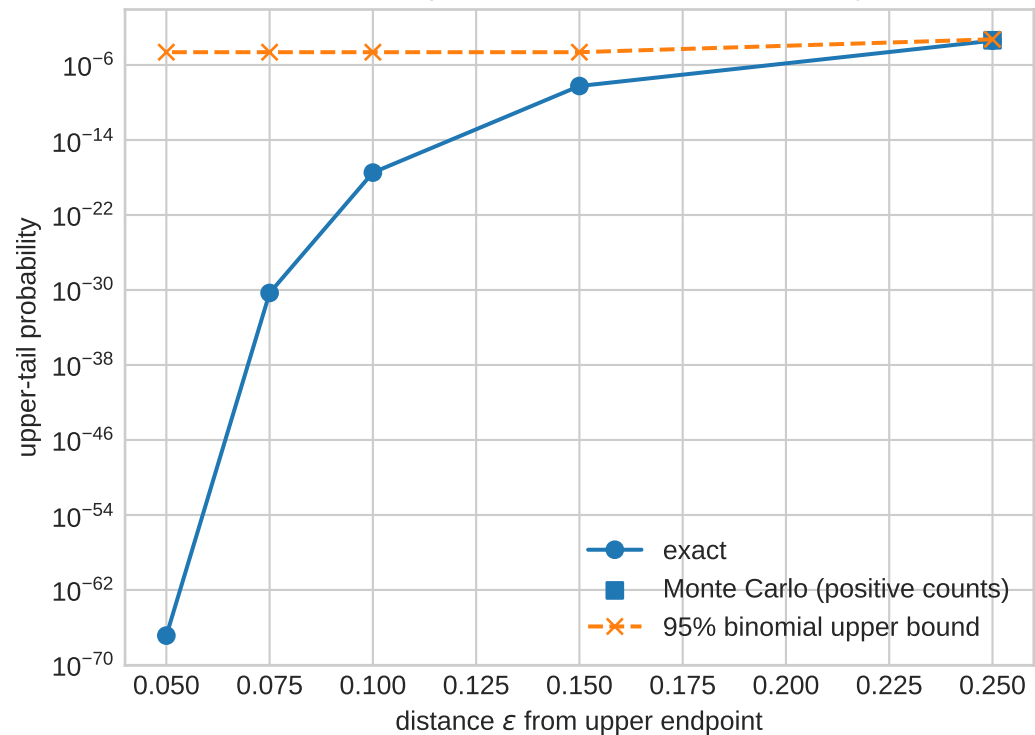
Finite endpoints encode Gaussian infinity
