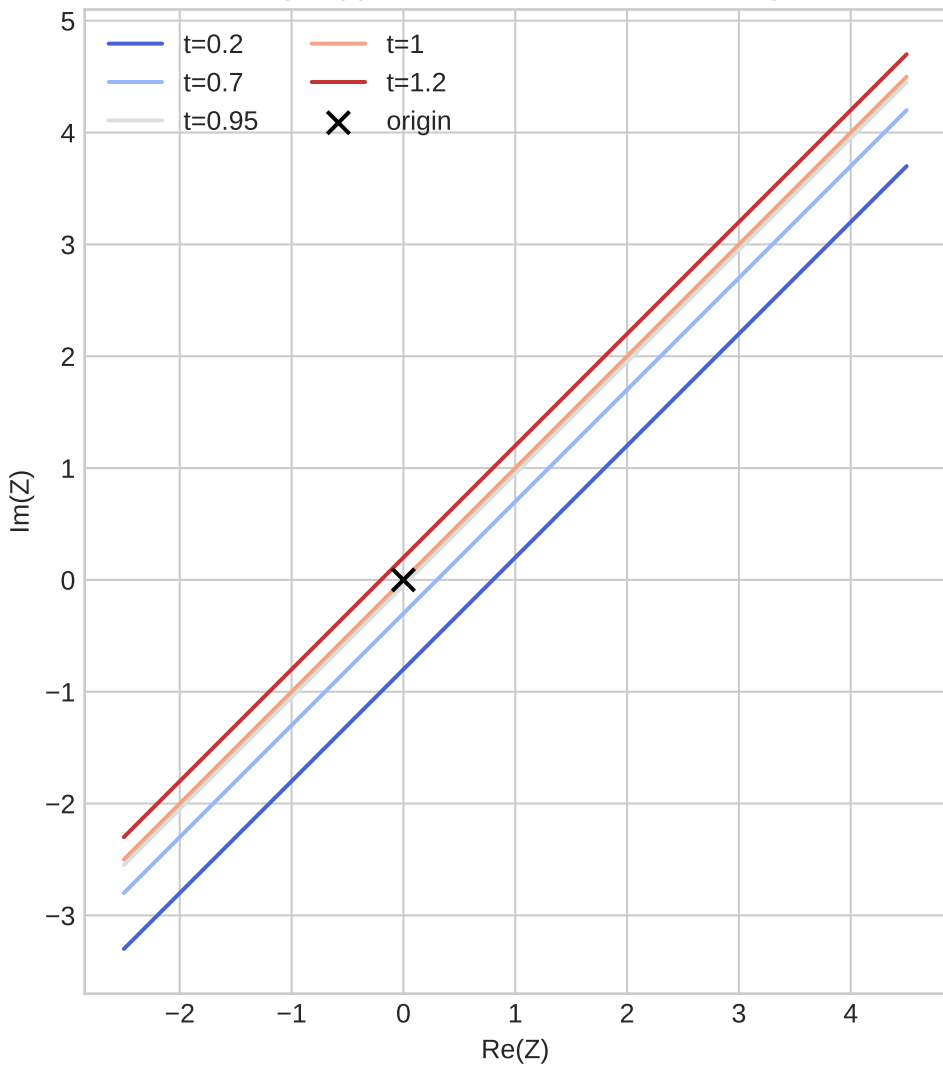
Moving support lines; the t=1 chart is singular
