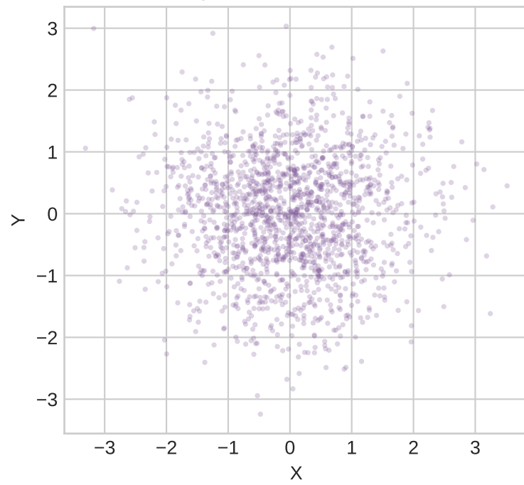
Two-driver planar Brownian law: rank two
