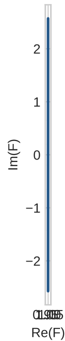
Secant coordinates: changing speed on a line
