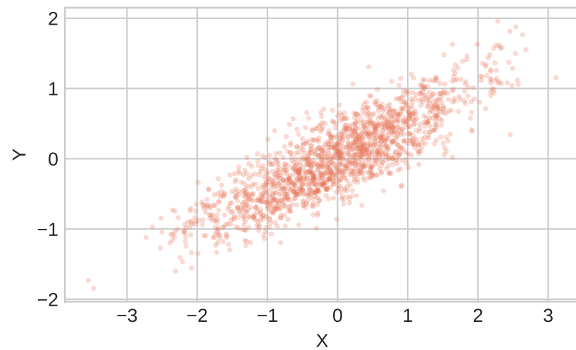
One driver, dY = Xdt : terminal rank two
