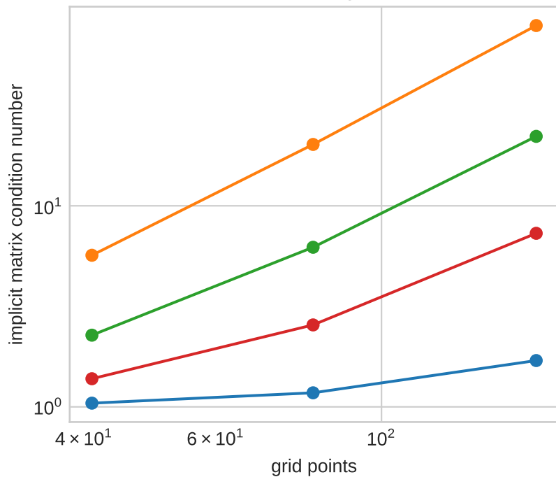
Bounded coordinates do not guarantee conditioning
