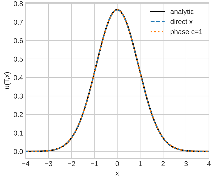
Same heat solution in two coordinates
