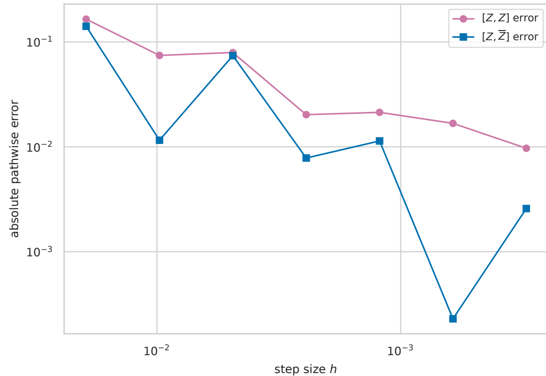
Discrete brackets approach distinct Itô targets
