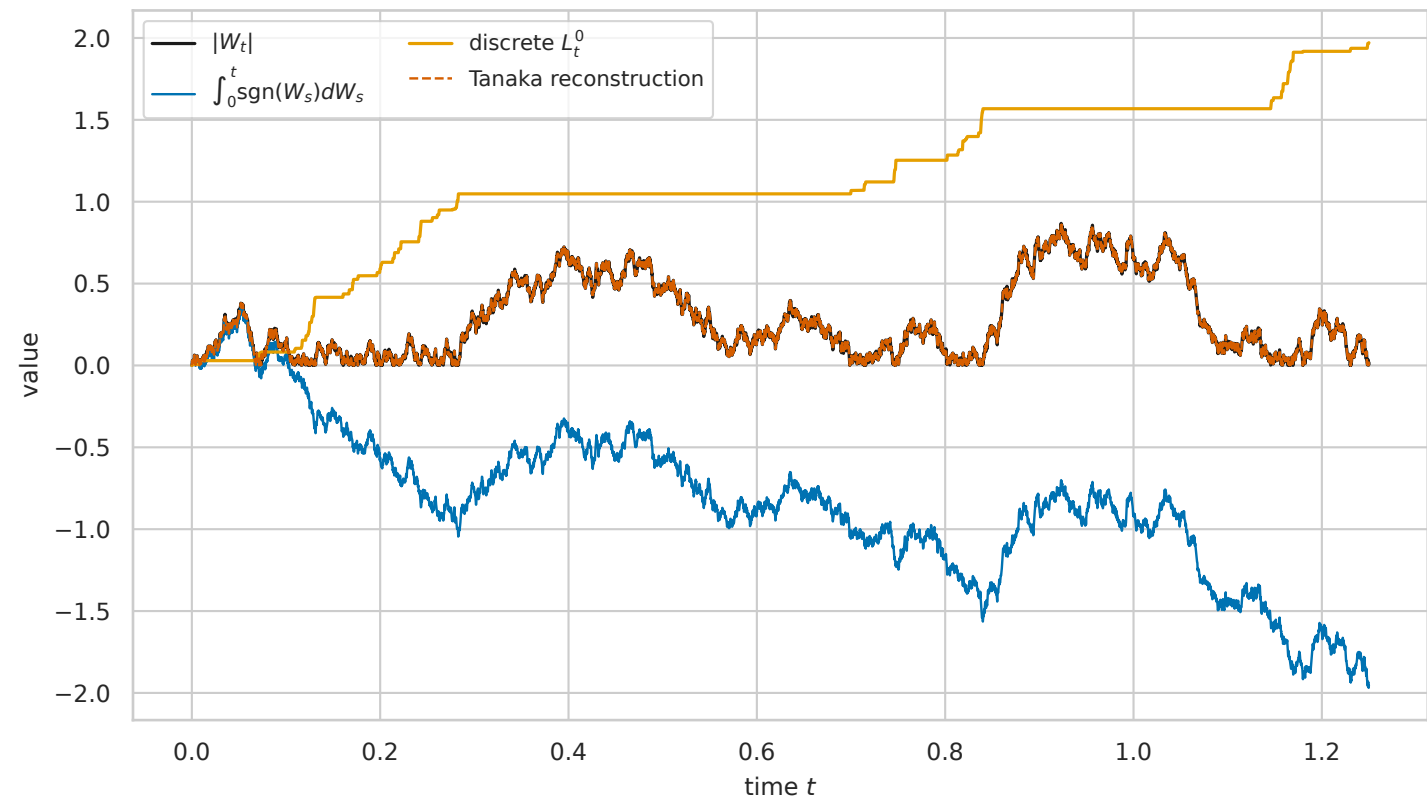
Tanaka decomposition on one grid
