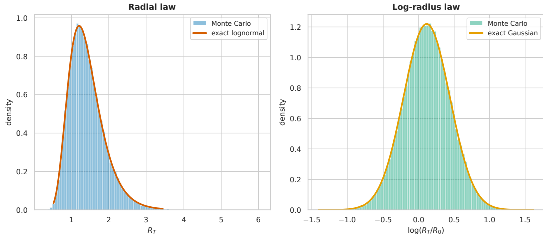
Figure 15: Monte Carlo histograms of radius and log-radius overlay their exact lognormal and Gaussian densities.
