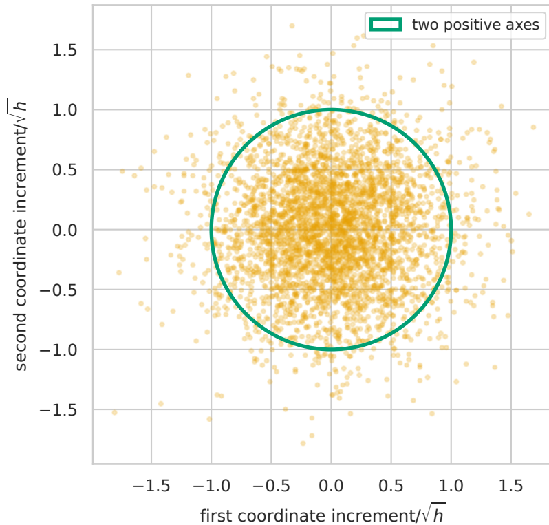
Two drivers: full-rank covariance ellipse
