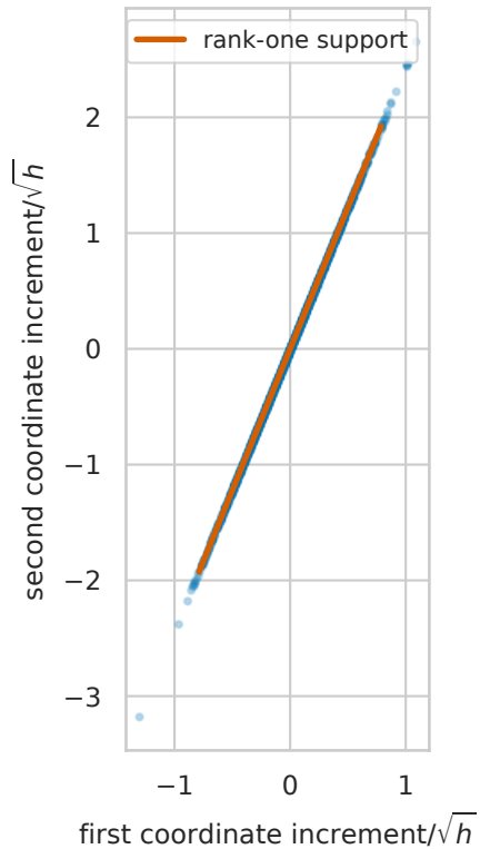
One driver: collapsed covariance ellipse
