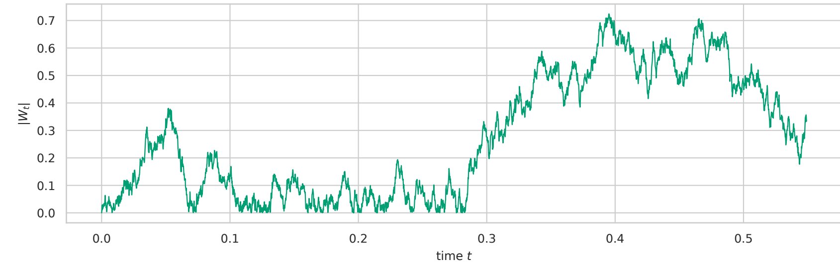
Reflection creates a nonsmooth radius at the origin
