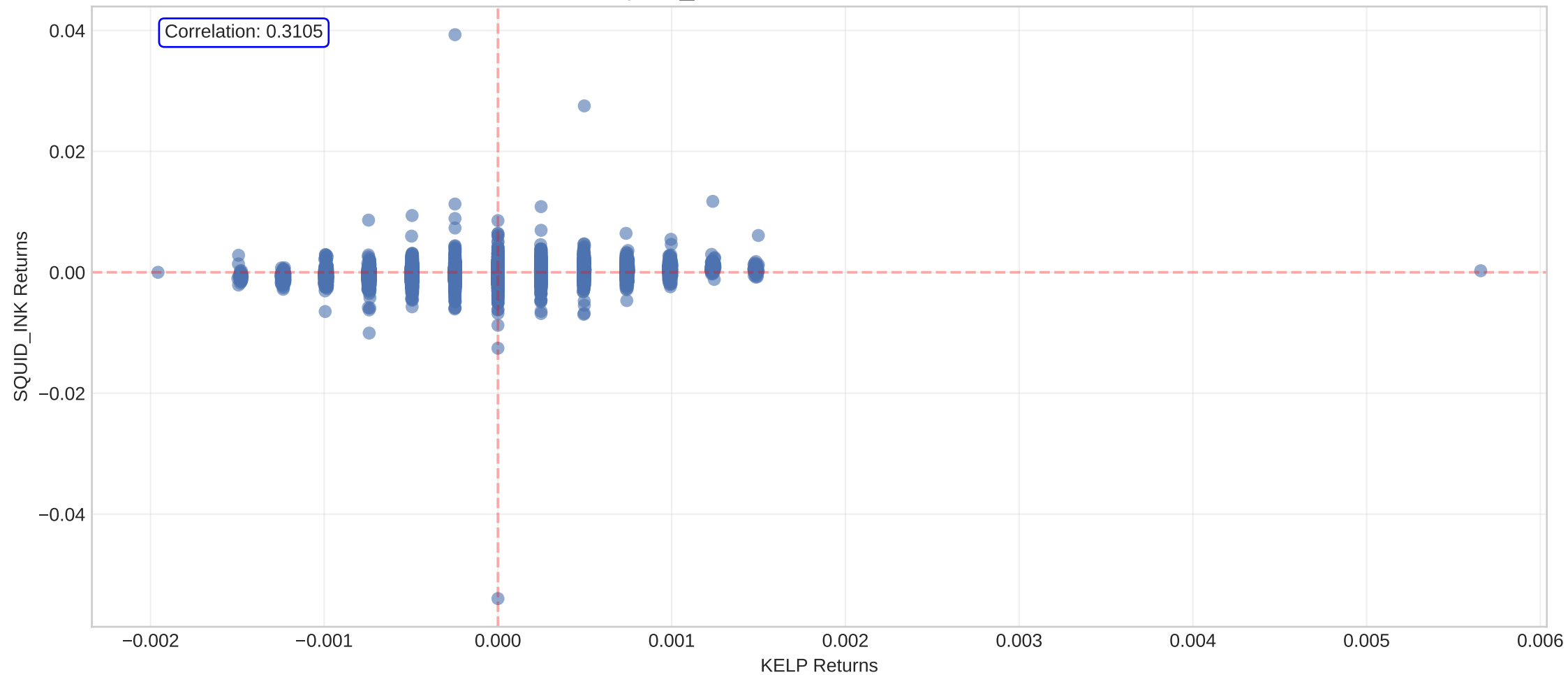
SQUID_INK Returns vs KELP Returns
