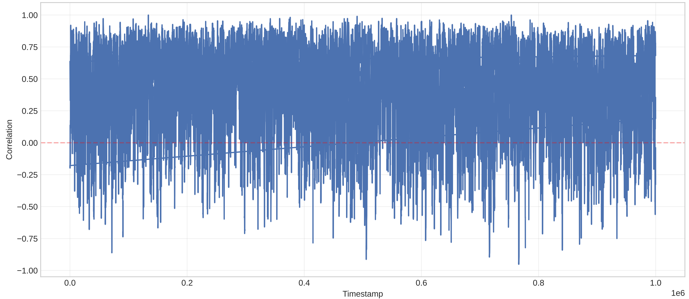
Rolling 10-period Correlation between SQUID_INK and KELP Returns
