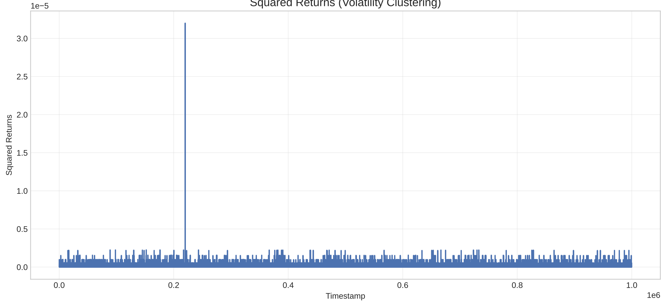
Squared Returns (Volatility Clustering)
