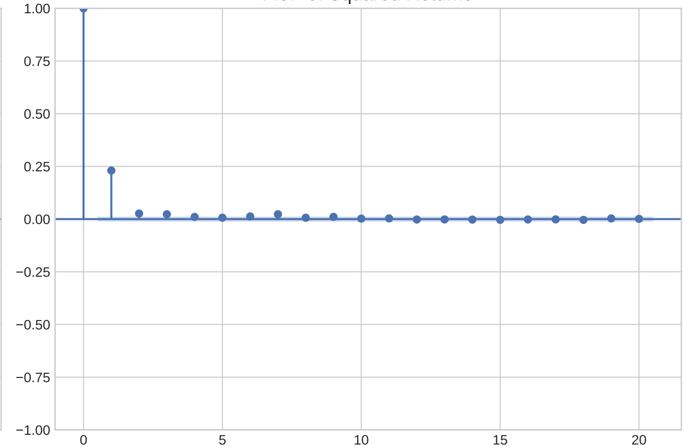
ACF of Squared Returns
