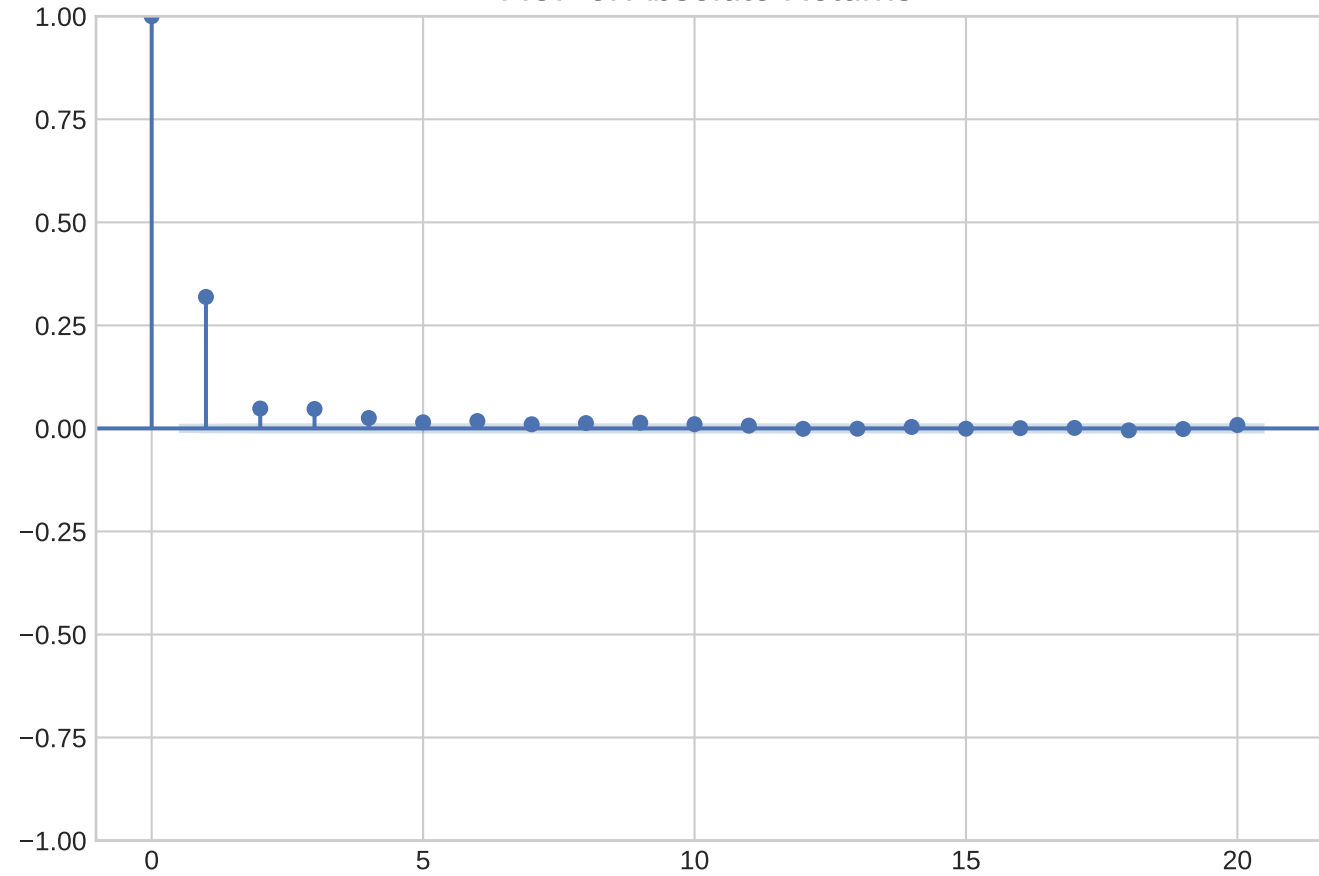
ACF of Absolute Returns
