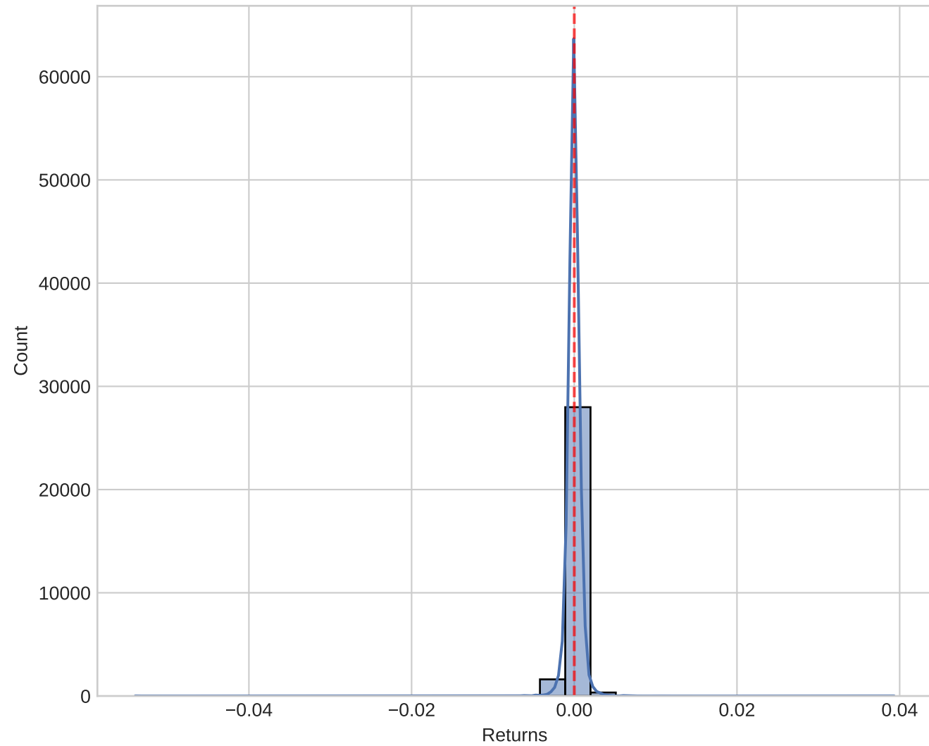
Distribution of squid_mid_ret Returns
