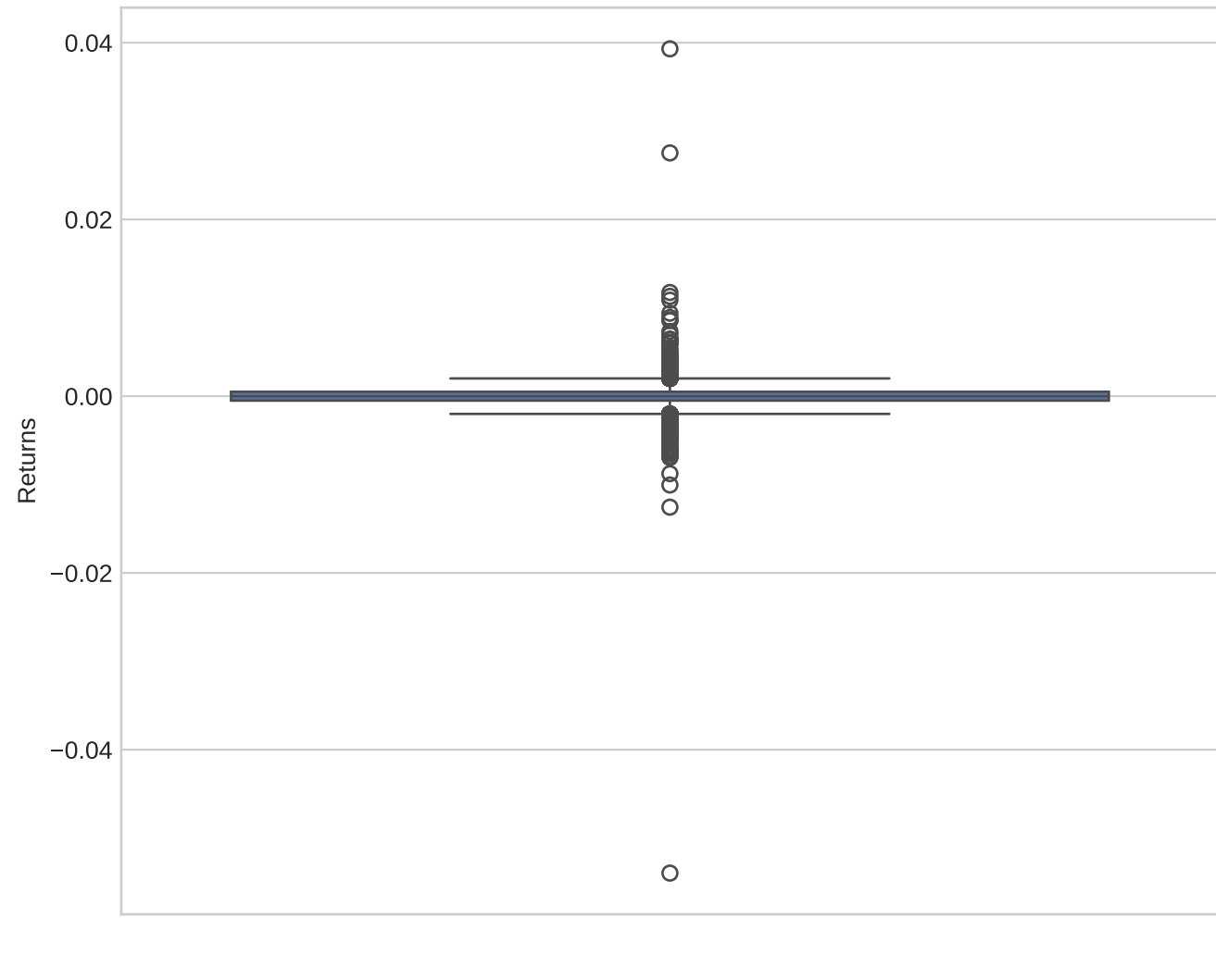
Box Plot of squid_mid_ret Returns
