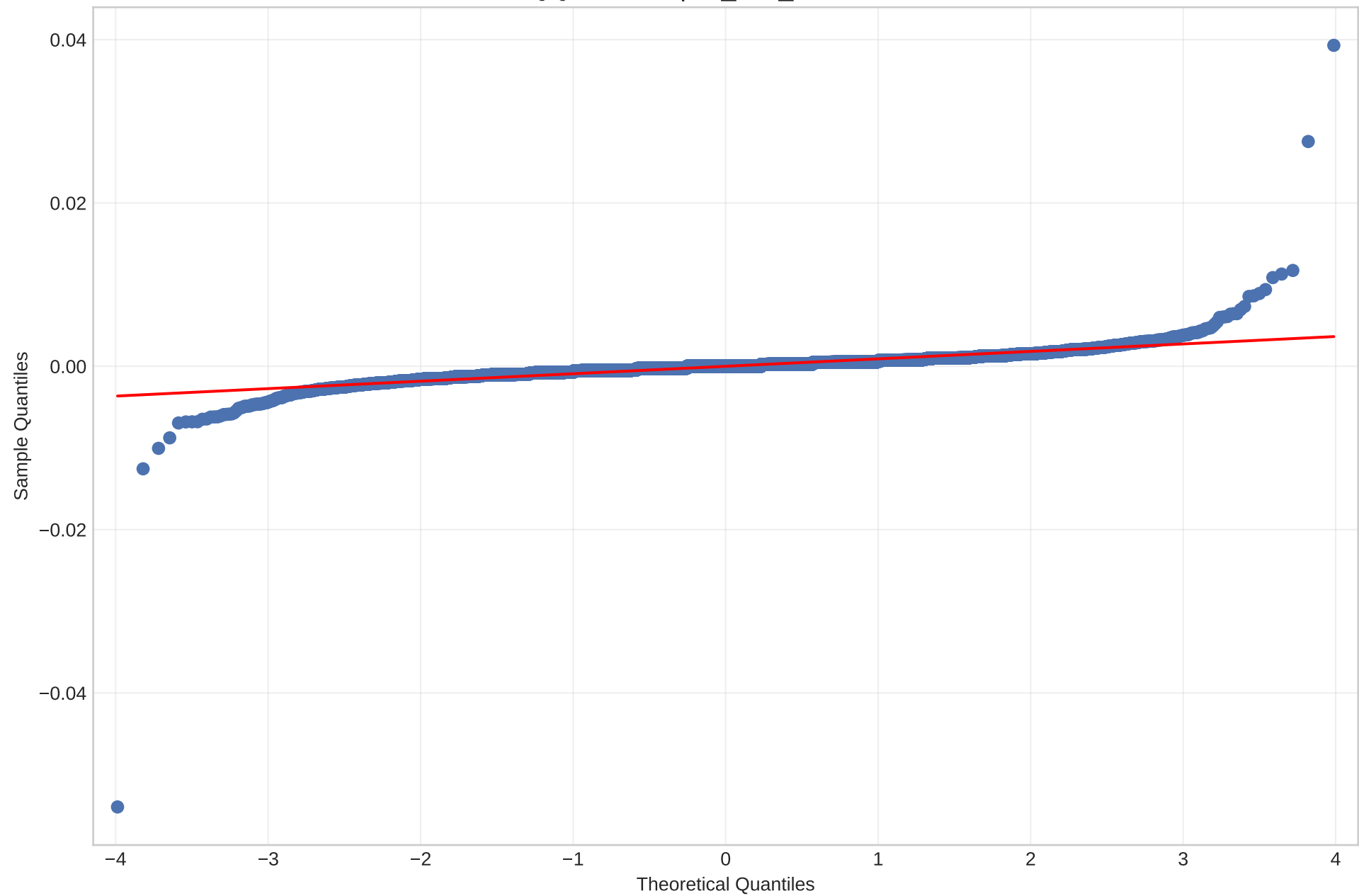
QQ Plot of squid_mid_ret Returns
