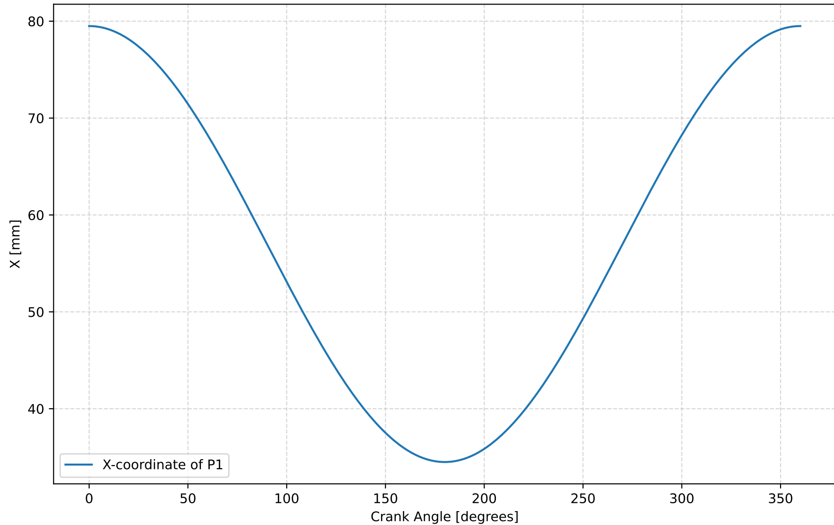
Figure 3: P1 x-Position vs. Crank Angle
