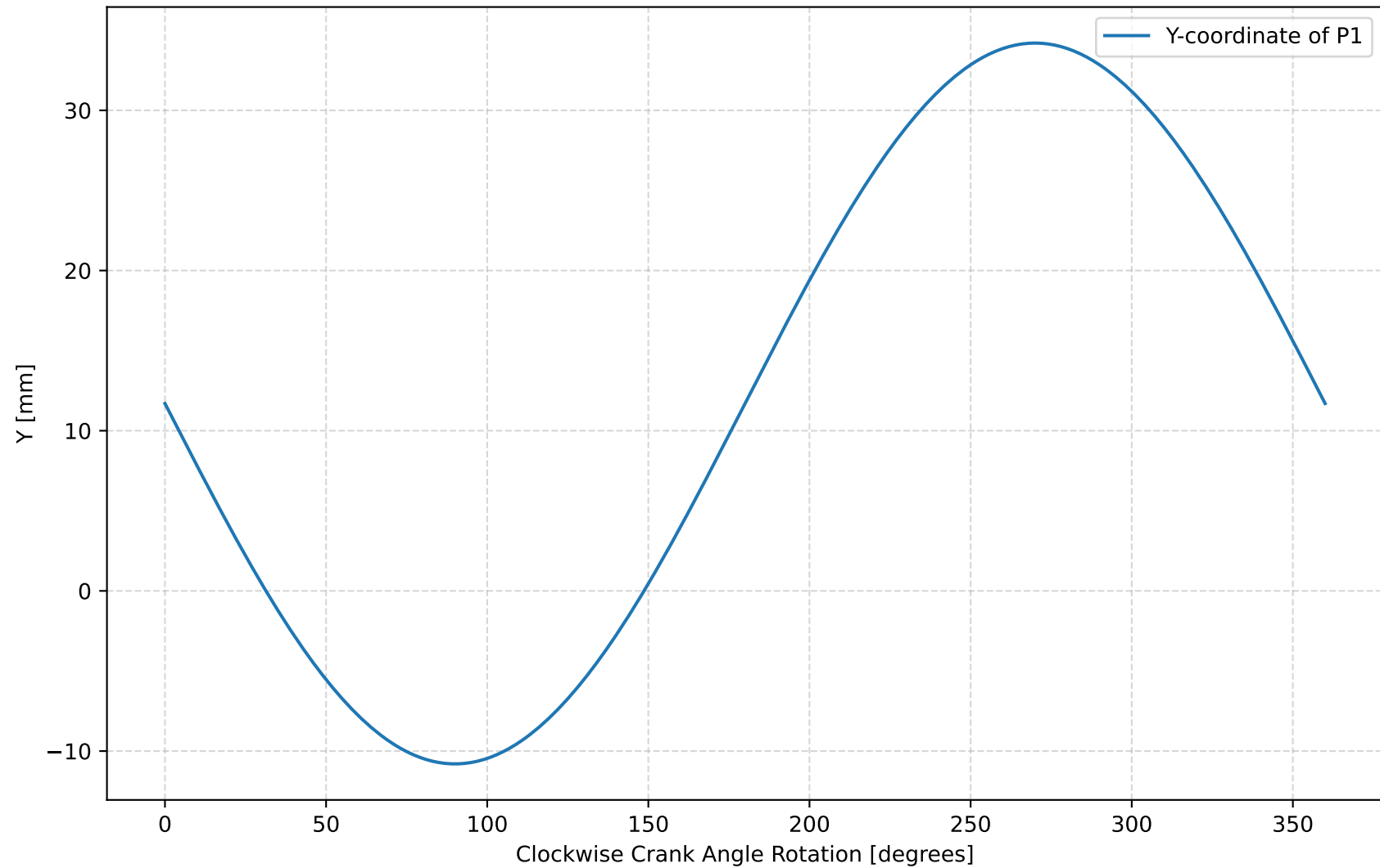
Figure 4: P1 y-Position vs. Crank Angle
