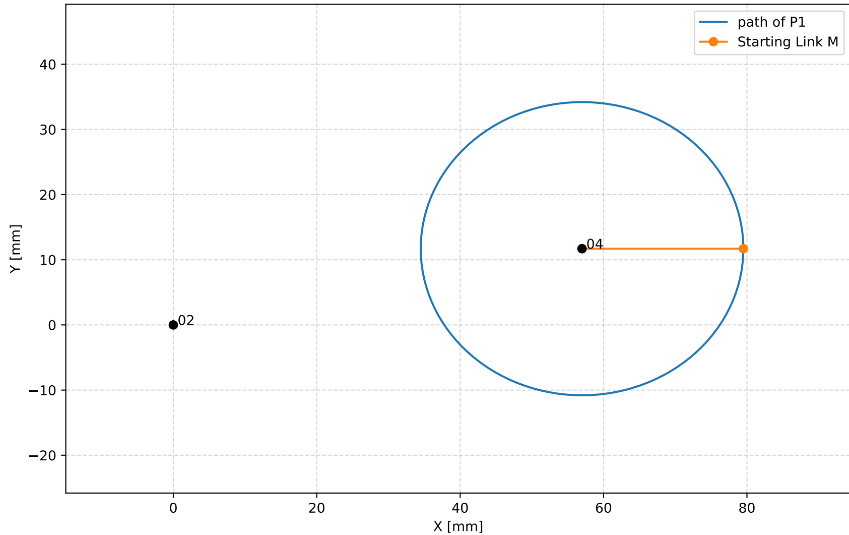
Figure 2: Point P1 Trajectory
