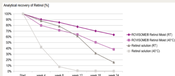
Figure 1: Improved stability of retinol.
