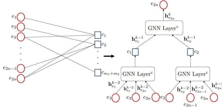
Figure 23: Example structure for decoding qLDPC codes (Figure 1[16])
