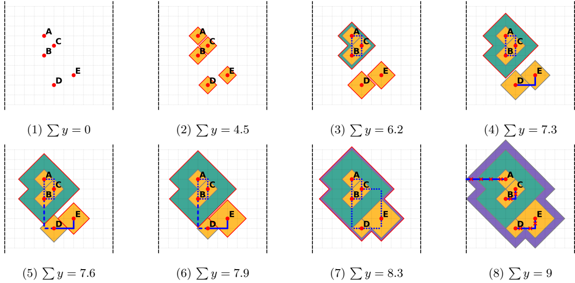
Figure 10: Figure 7, from [31], highlighting the blossom algorithm for an unweighted decoding graph. In the final stage, the nonzero dual variables are y_A = y_B = y_C = y_D = 1 , y_E = 2 , y_{ABC} = 2 , y_{ABCDE} = 1 . Dual variables corresponding to other odd subsets of vertices (such as y_{BDE} ) are zero.
