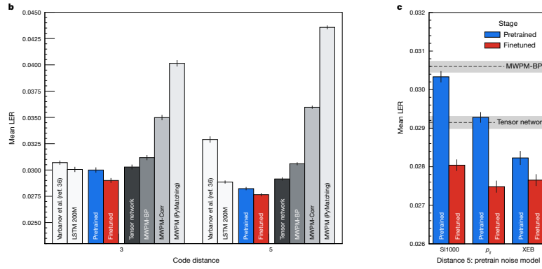
Figure 29: LERs of decoder, before and after fine-tuning on Sycamore experiments (Figure 3)
