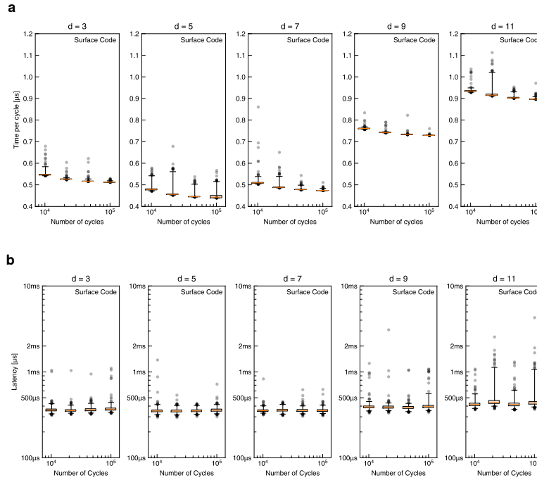
Figure 39: Latency and throughput experiments for AlphaQubit 2 (Figure S11)
