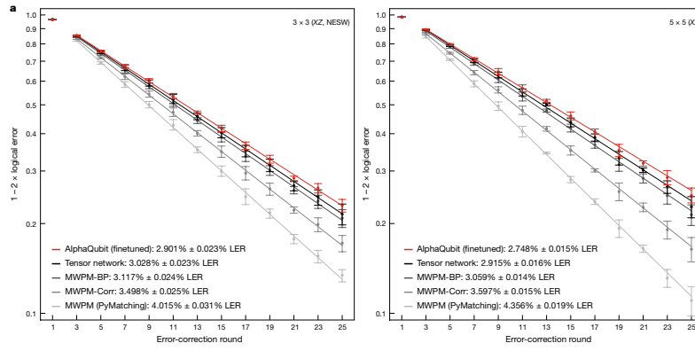
Figure 28: Logical error per round on 3 × 3 and 5 × 5 Sycamore experiment (Figure 3)
