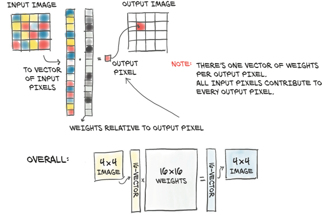
Figure 14: Treating an image like an array of numbers increases the number of required parameters (Figure 7.15 of [22]).
