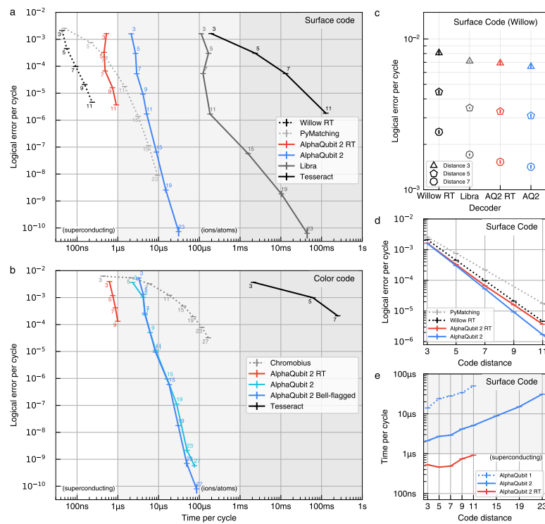
Figure 38: Decoding Throughput comparison (Figure 4)
