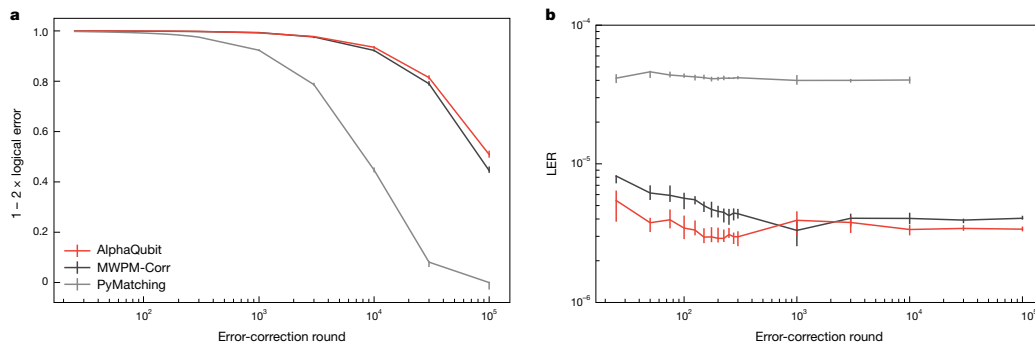
Figure 34: Comparison of AlphaQubit, MWPM-Corr and MWPM (Pymatching) on large number of error correction rounds. (Figure 4)
