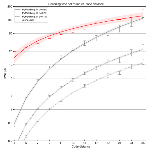
Figure 35: Decoding throughput vs code distance (Extended data Figure 7)
