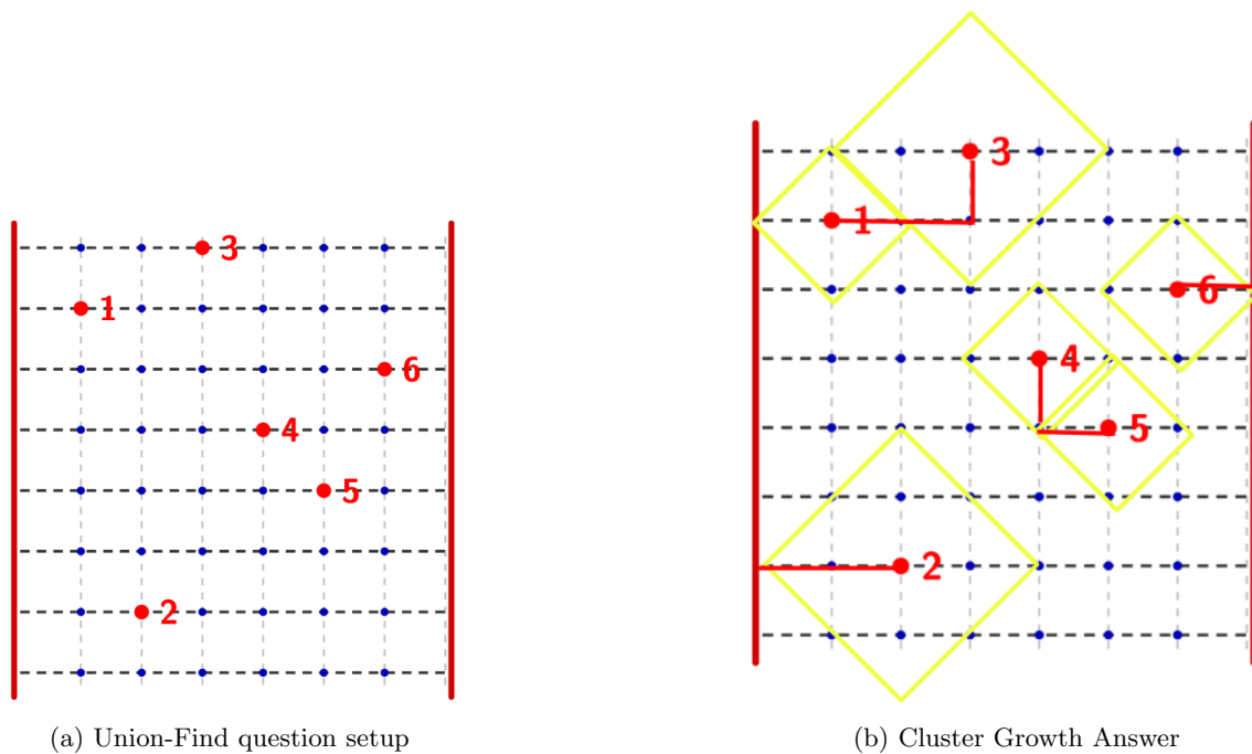
Figure 9: Quiz Question 2
