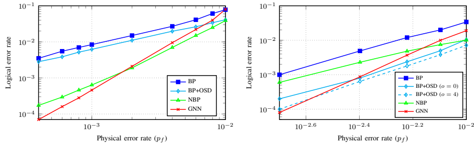
Figure 24: Decoding LER for example of [16] on hypergraph (left) and bicycle (right) codes (Figs. 2, 3[16])
