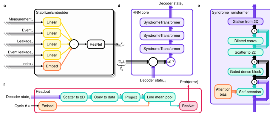
Figure 31: Details of Embedder and RNN core (Extended Data Figure 4)
