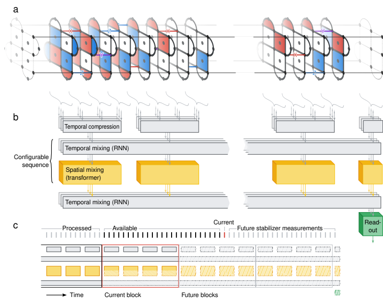
Figure 36: Overview of AlphaQubit 2 for surface-code decoding (Figure 1)
