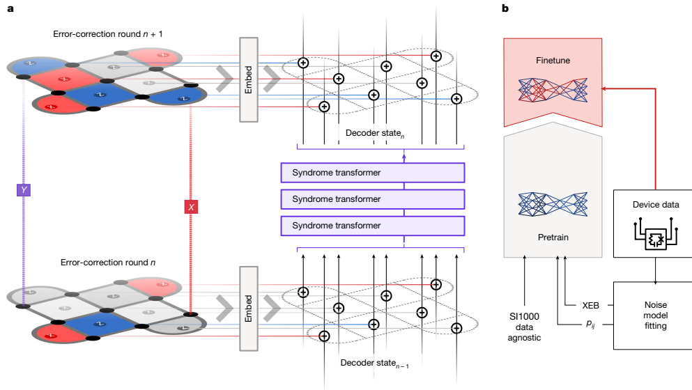
Figure 26: Overview of training method for AlphaQubit 1 (Figure 2)
