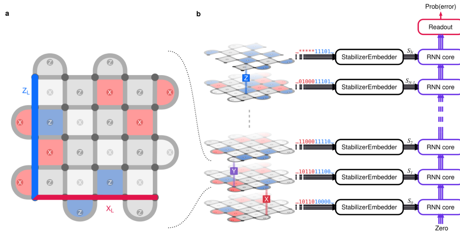
Figure 27: Architecture outline of AlphaQubit 1 (Extended Data Figure 4)
