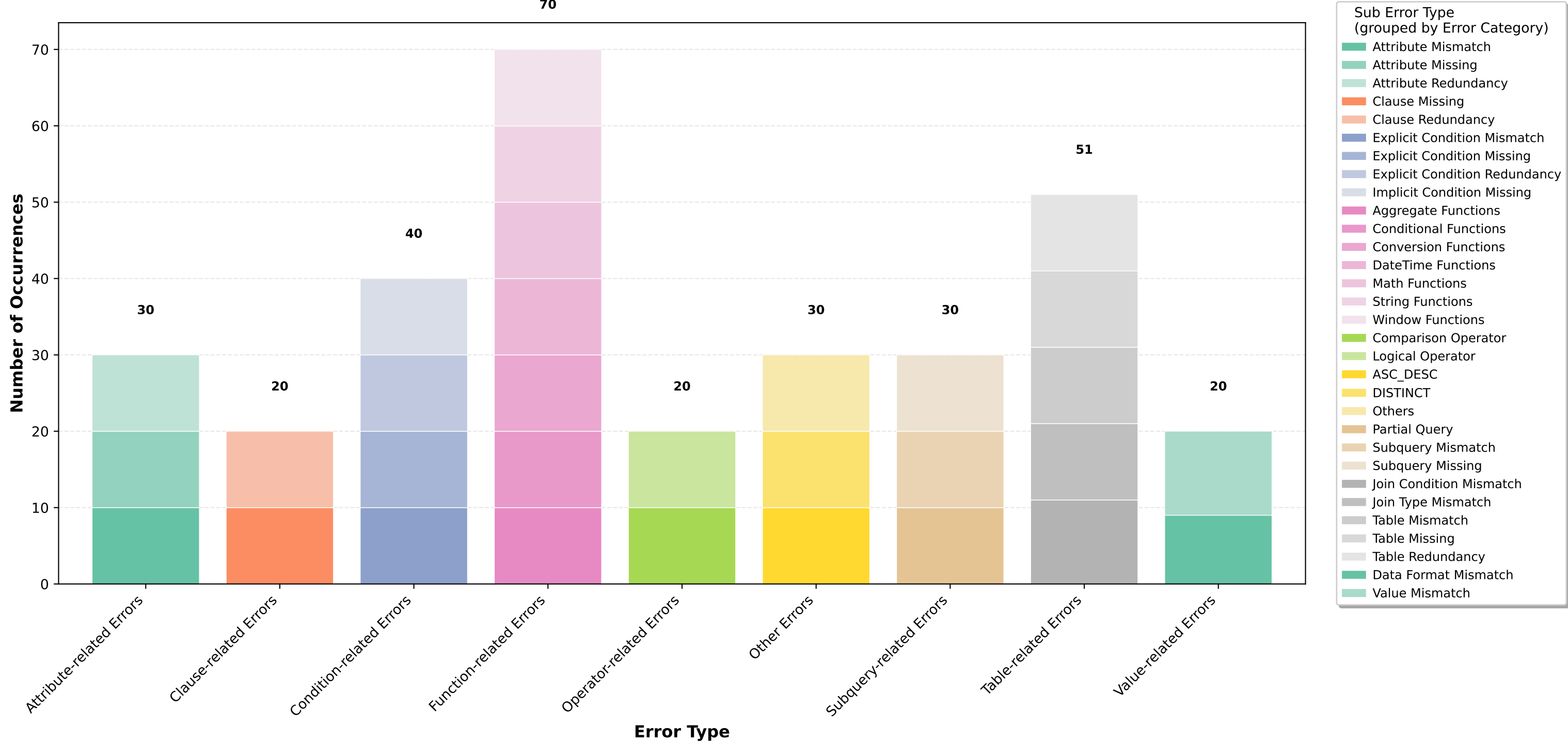
Distribution of Semantic Error Types and Subtypes
