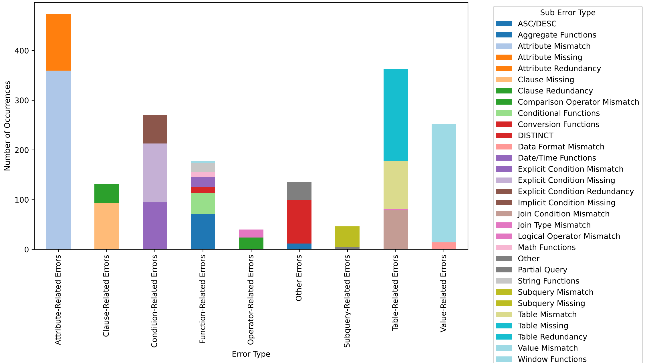
Distribution of Semantic Error Types and Subtypes (label == false)
