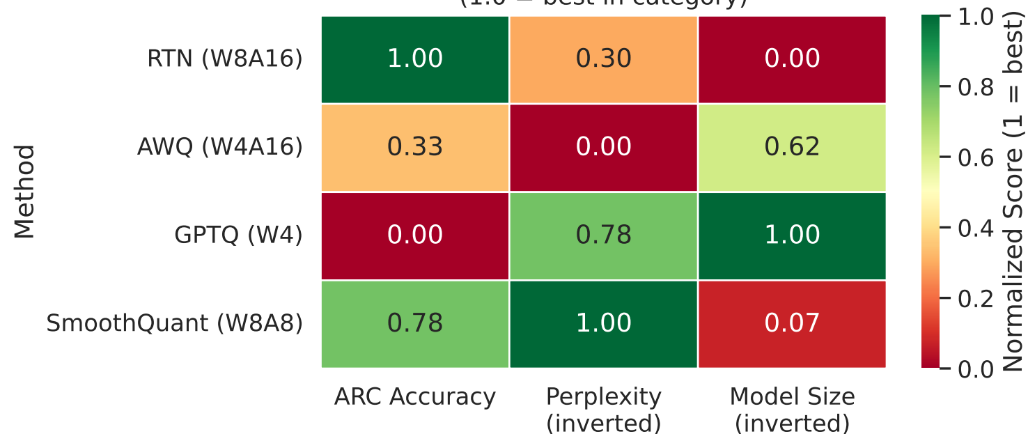
Full-Model Quantization — Normalized Method Comparison (1.0 = best in category)
