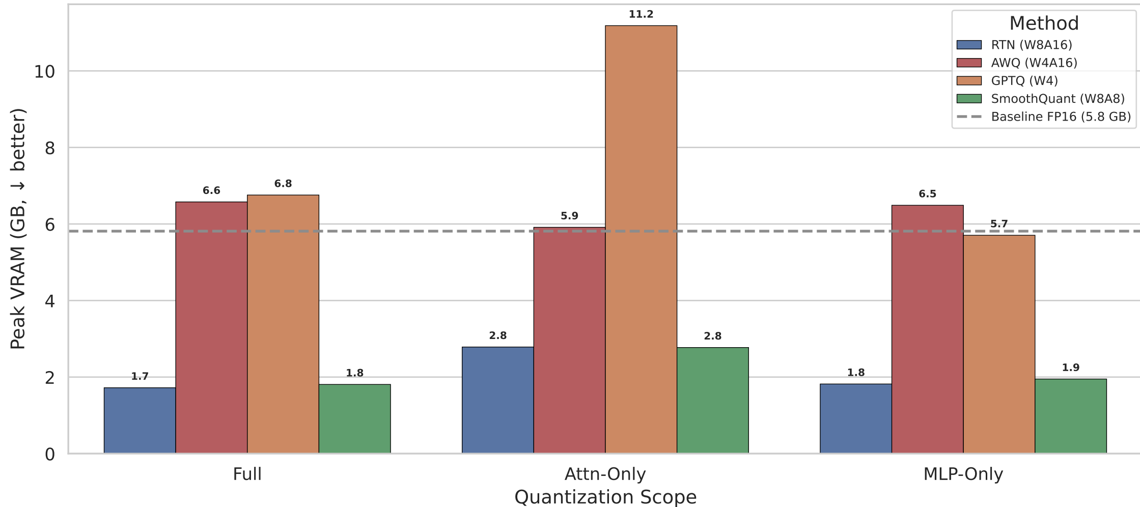
Peak VRAM Usage by Method × Scope (RTN/SmoothQuant achieve lowest VRAM; GPTQ Attn-Only anomalously high)
