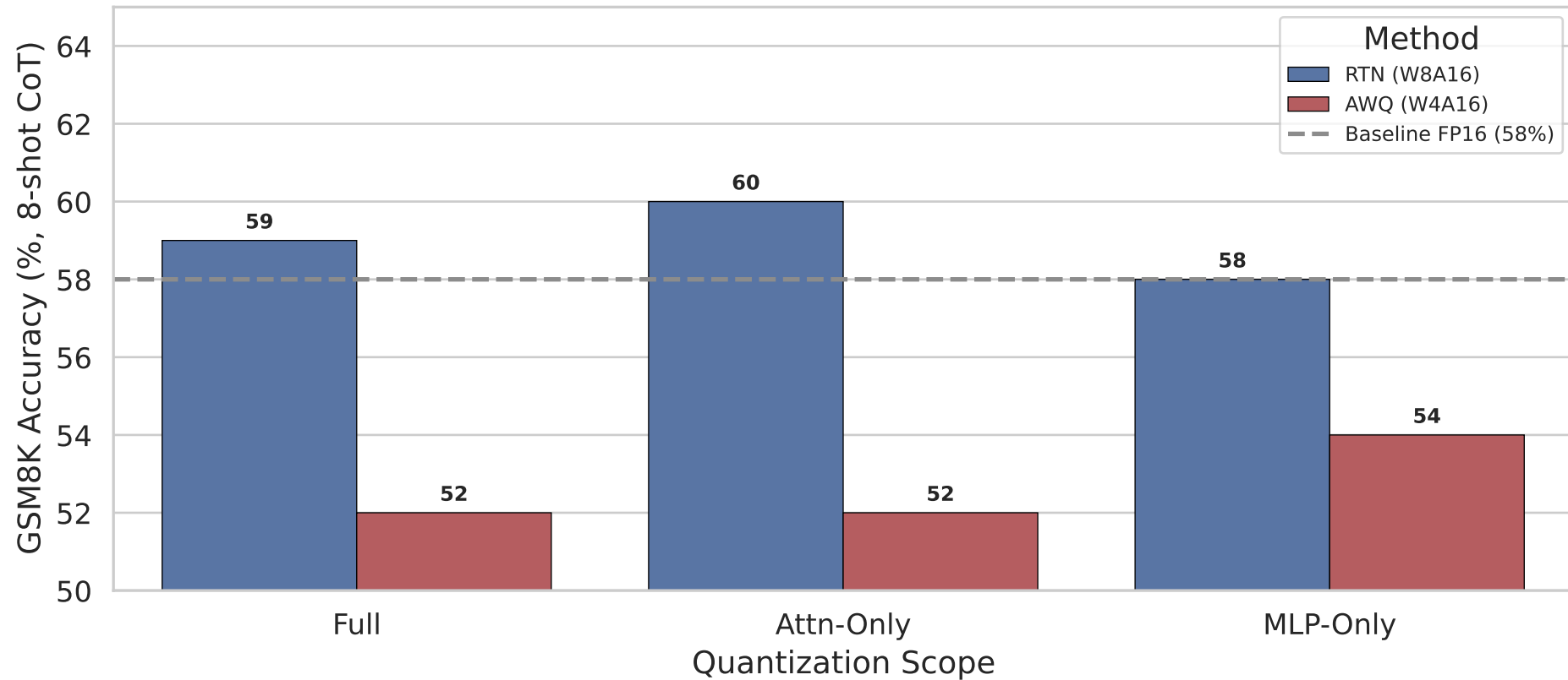
GSM8K Math Reasoning: RTN vs AWQ (8-shot chain-of-thought, Qwen2-1.5B)
