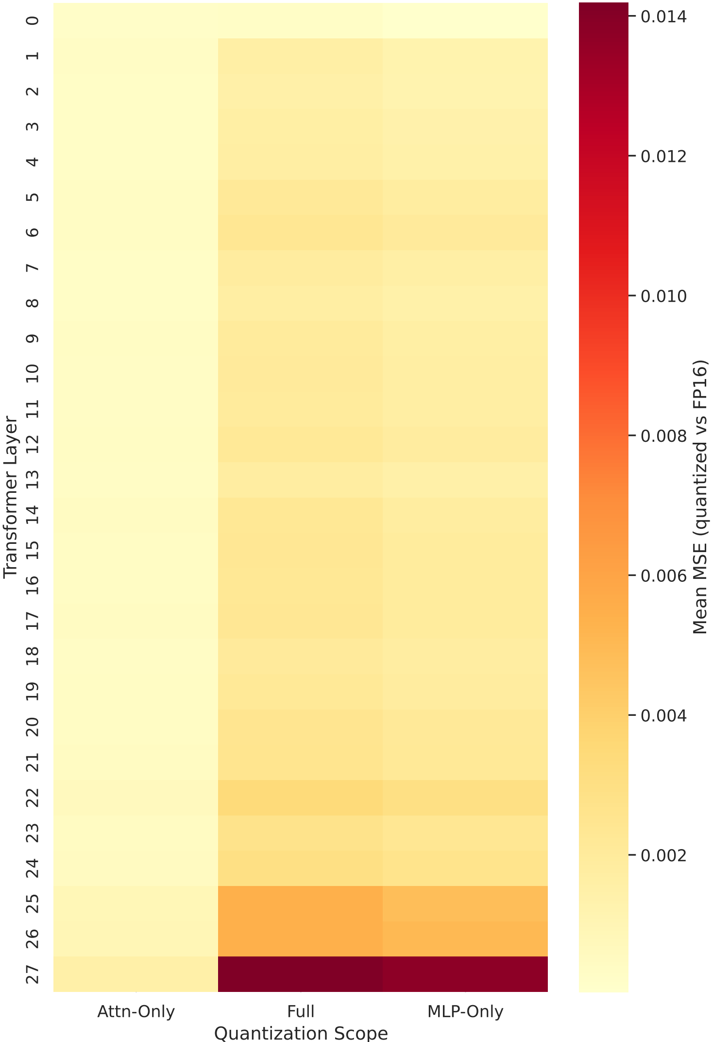
RTN (W8A16) — Per-Layer Mean MSE Heatmap (higher = more quantization error)
