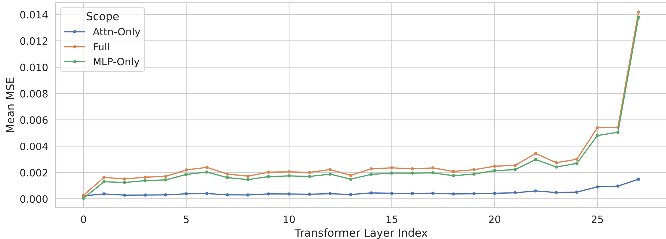
RTN (W8A16) — Layer-wise Quantization Error (spikes indicate sensitive layers — consistent with Dettmers et al., 2022)
