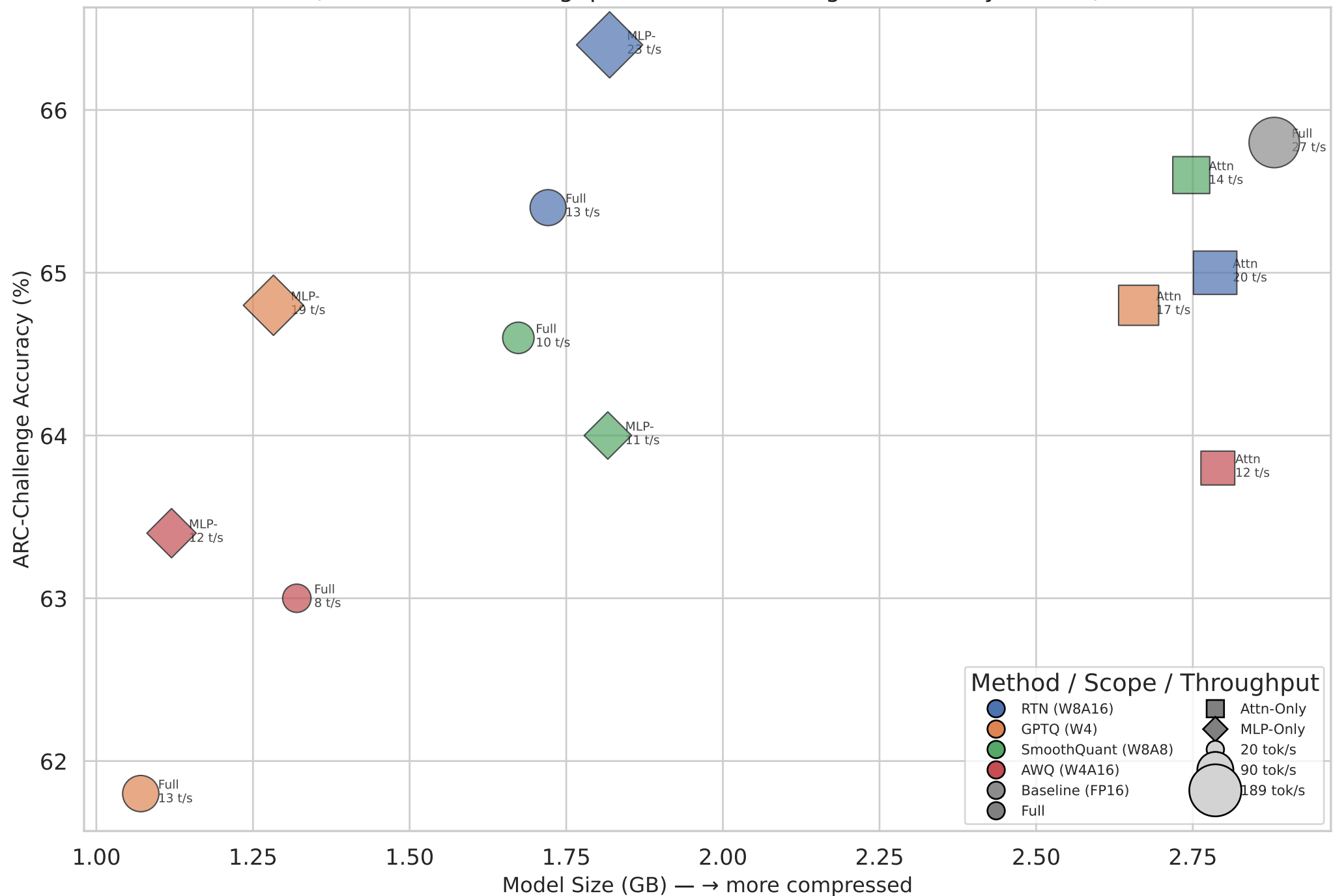
Compression-Accuracy-Throughput Trade-off (bubble size \propto throughput; lower size + higher accuracy is ideal)
