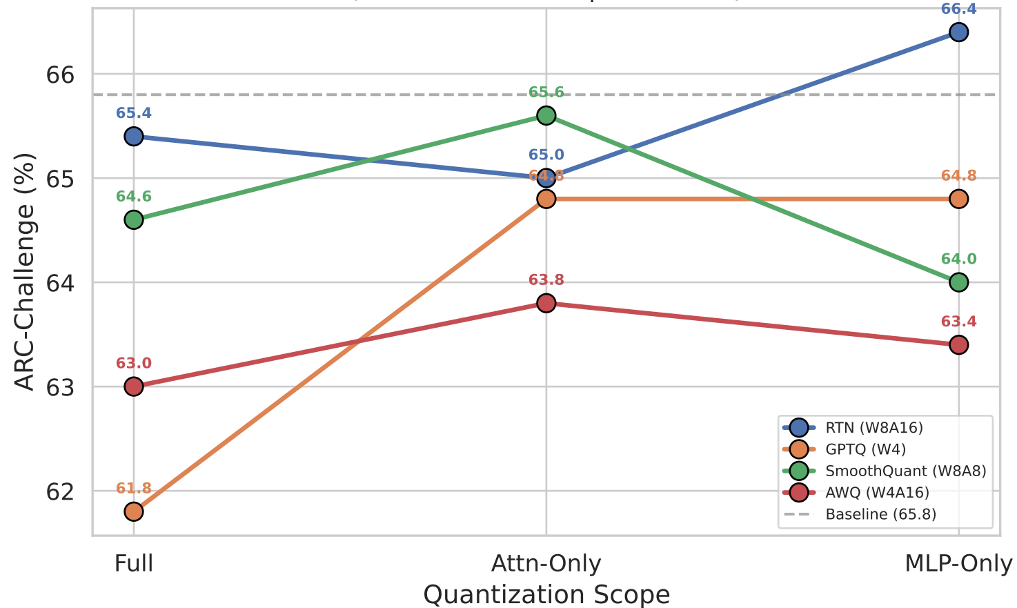
ARC-Challenge Accuracy by Scope (flat = robust to scope selection)
