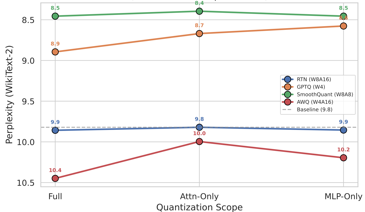
Perplexity by Scope (flat = robust to scope selection)
