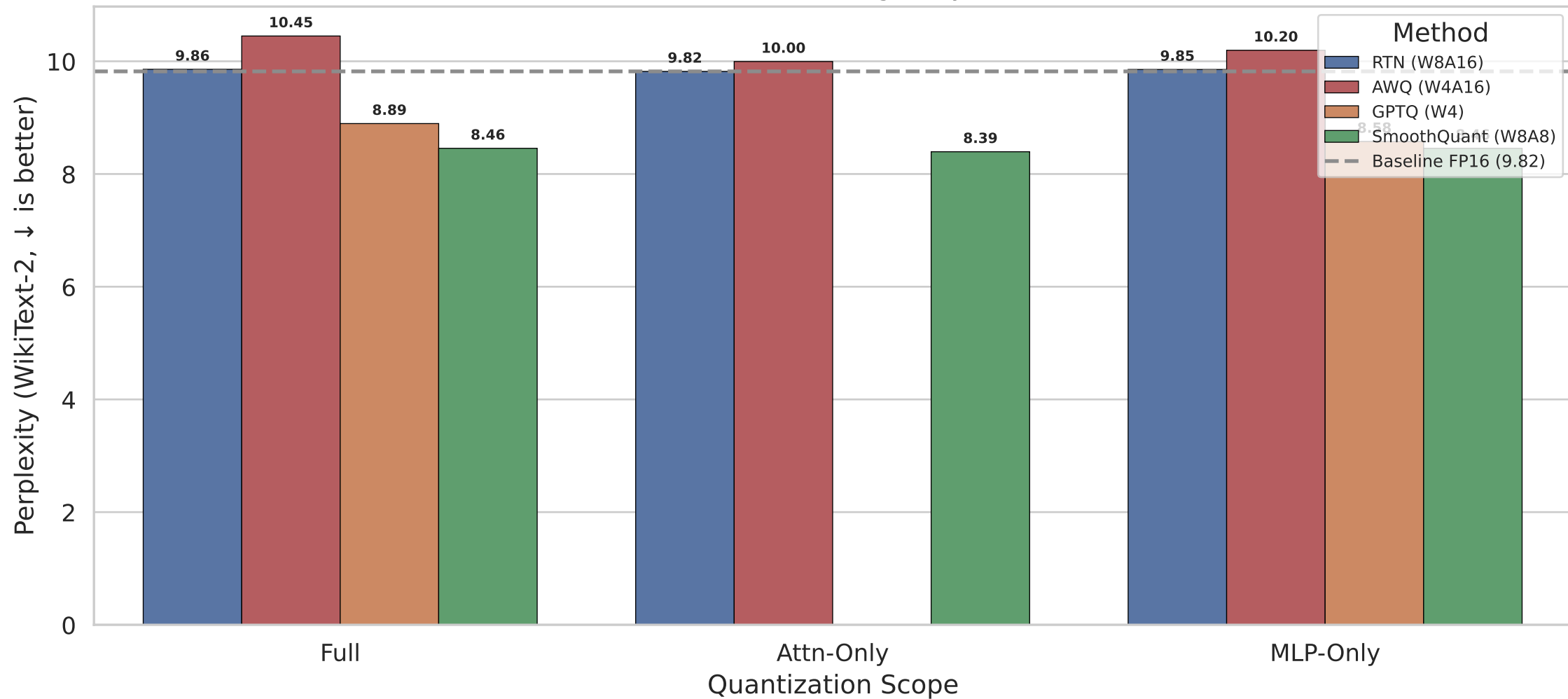
WikiText-2 Perplexity by Method × Scope (Qwen2-1.5B — note: eval configs vary across methods)
