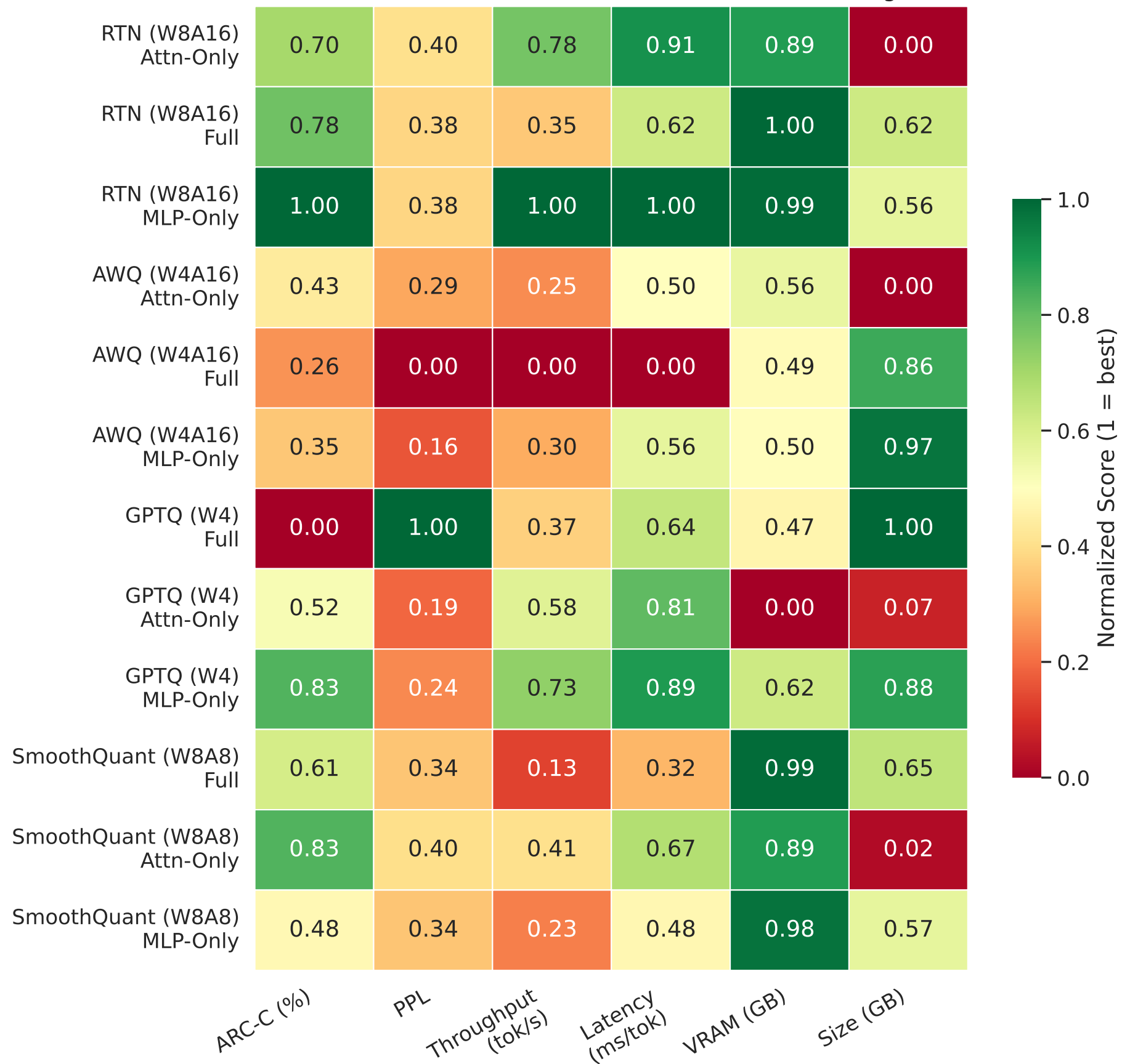
Multi-Metric Quantization Scorecard (all metrics normalized: 1.0 = best across all configs)
