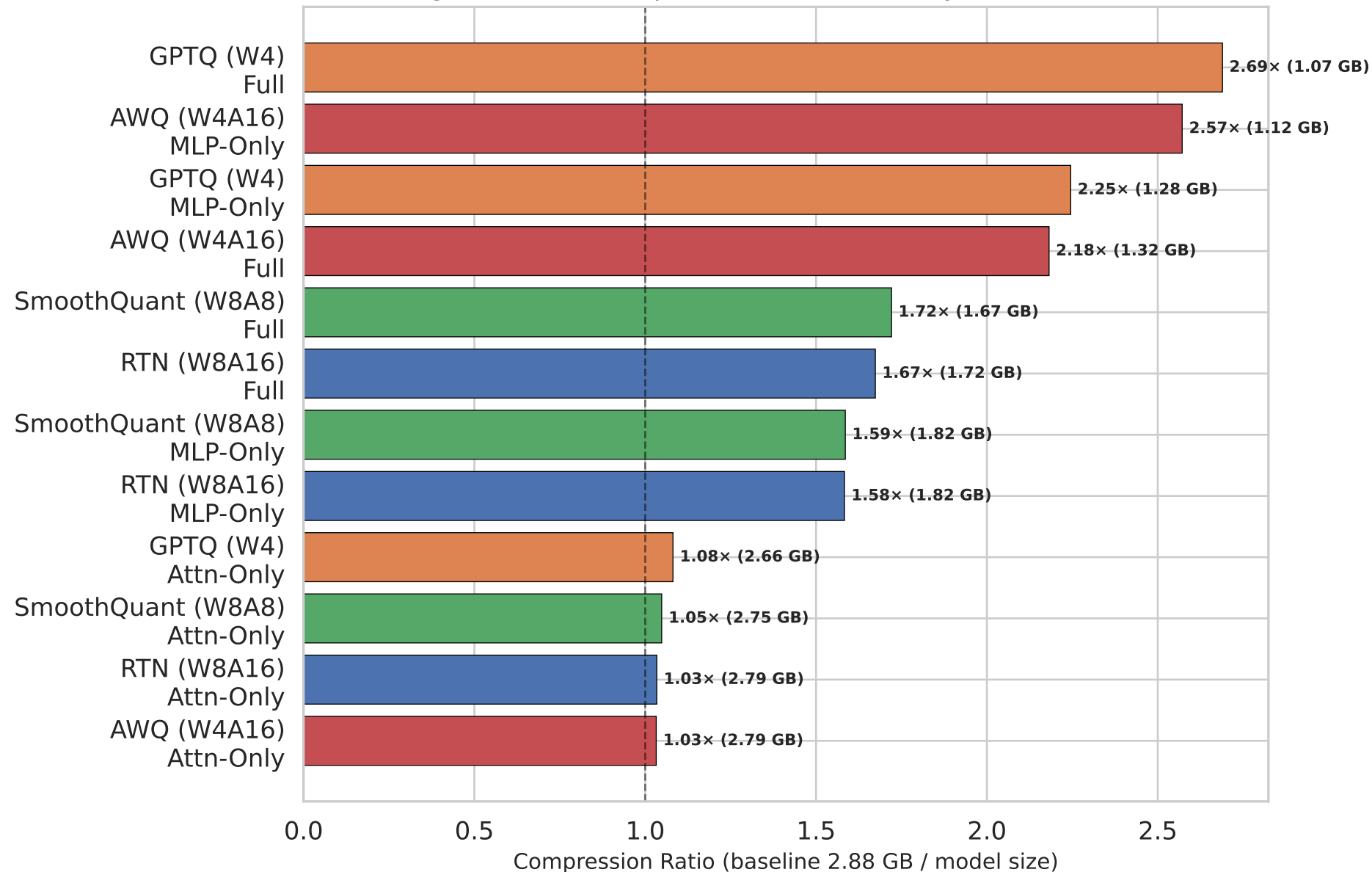
Model Compression Ratio by Configuration (higher = more compressed; AWQ MLP-Only achieves 2.57×)
