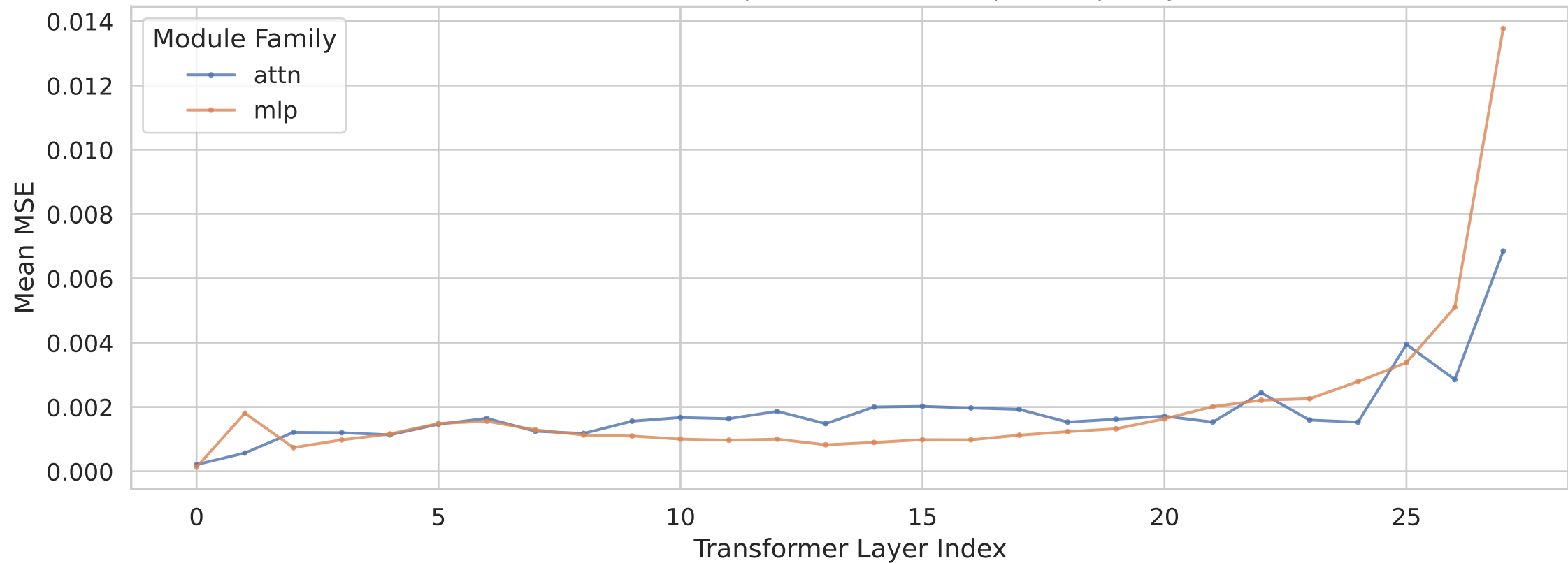
RTN — Attention vs MLP Module MSE by Layer (identifies which component is harder to quantize per layer)
