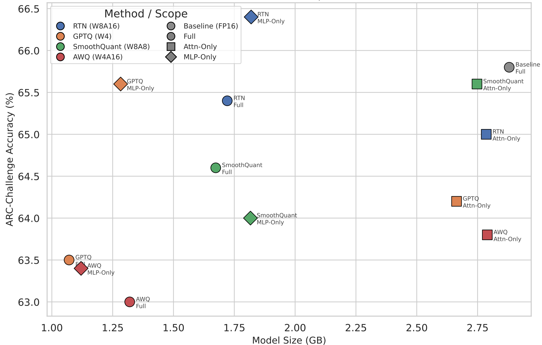
Model Size vs. ARC-Challenge Accuracy (Qwen2-1.5B, 500 samples, 0-shot)
