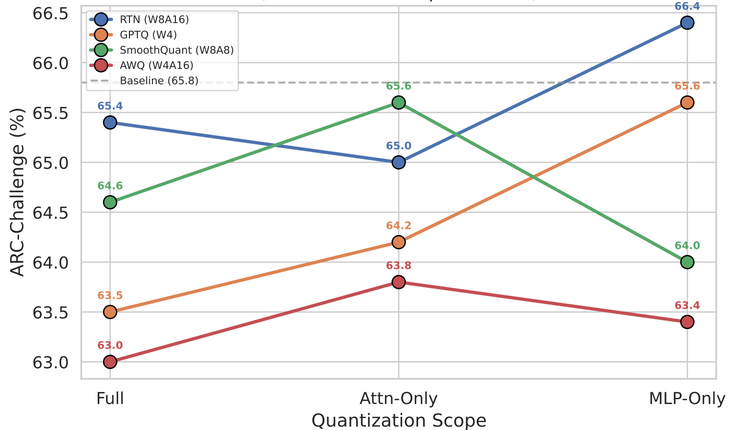
ARC-Challenge Accuracy by Scope (flat = robust to scope selection)
