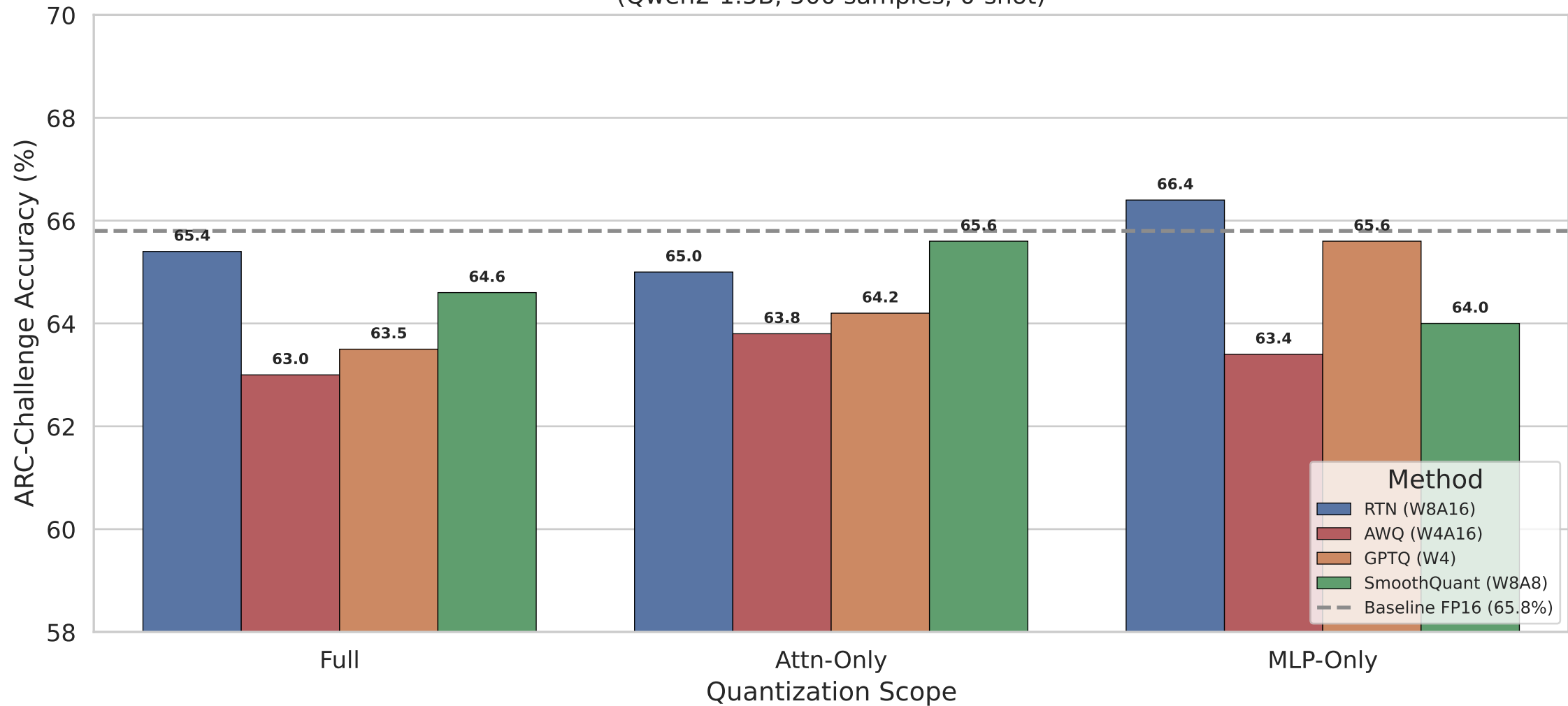
ARC-Challenge Accuracy: Quantization Method × Scope (Qwen2-1.5B, 500 samples, 0-shot)
