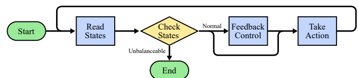
Figure 1. Flowchart of basic balancing logic. After turning on, the robot keeps reading its state, such as the pitch angle or the angular velocity of y-axis. If it's not strongly unbalanced, feedback controllers are used to generate an output from the state. The output is used to control the robot, such as moving forward or turn left. The feedback loop can balance the robot theoretically.
