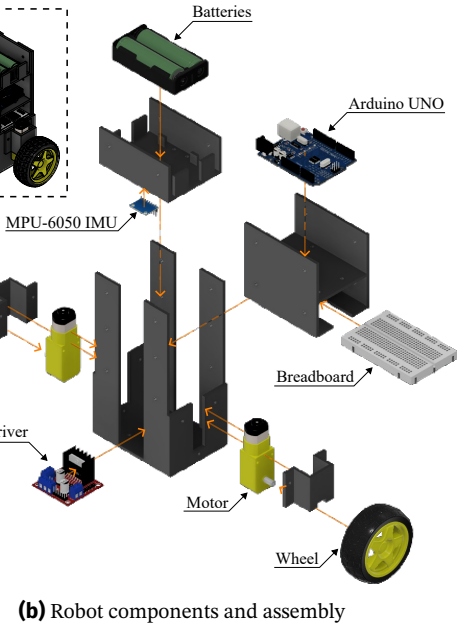
Figure 4. A chassis model design.
