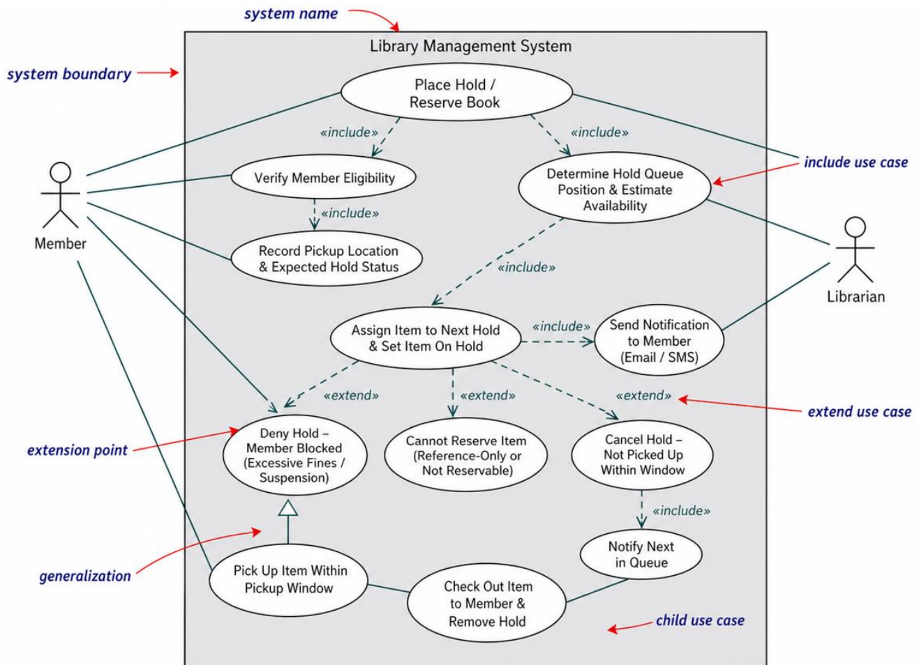
Figure 8: Reserve Book
