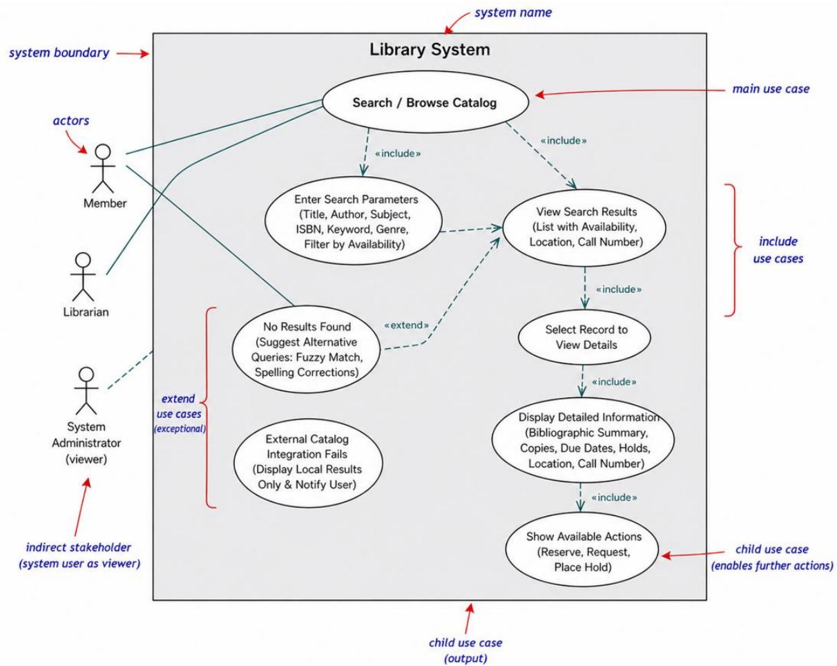
Figure 2: Browse Catalog
