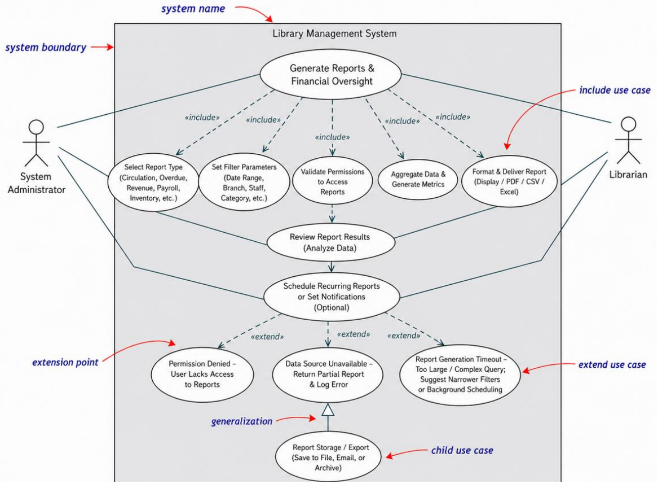
Figure 4: Generate Report
