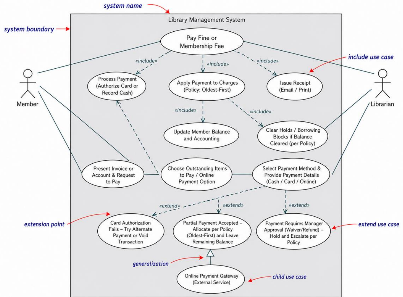
Figure 5: Pay Fine
