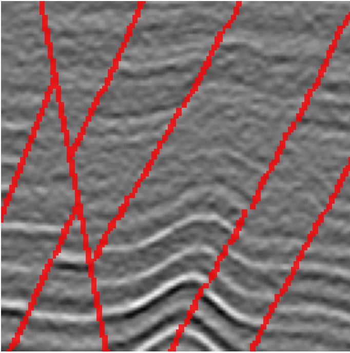
Wu Synthetic — Fault Overlay Slice X=64 (inline)
