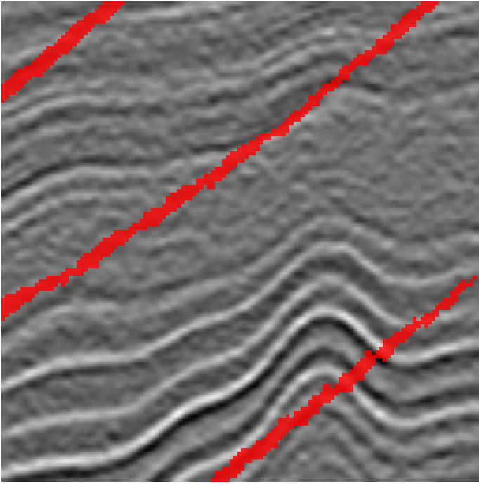
Wu Synthetic — Fault Overlay Slice Y=64 (crossline)
