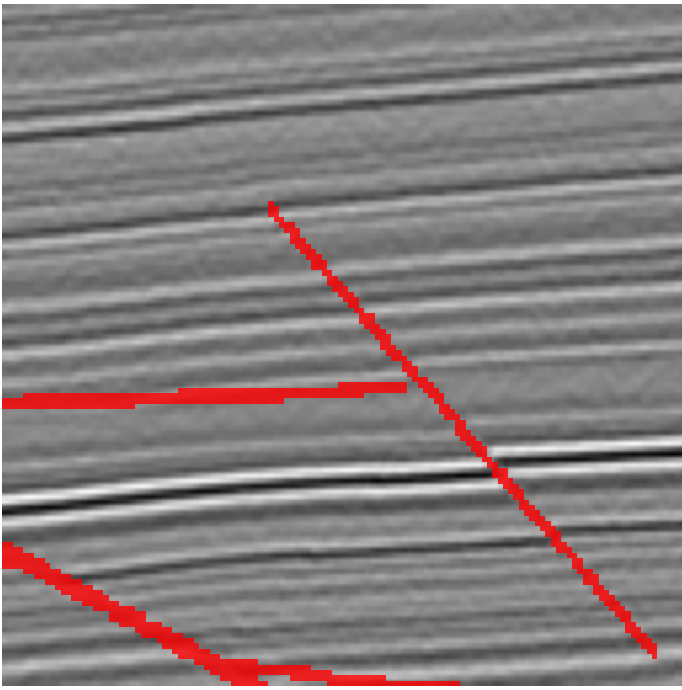
GRvA Synthetic — Fault Overlay Slice X=64 (inline)
