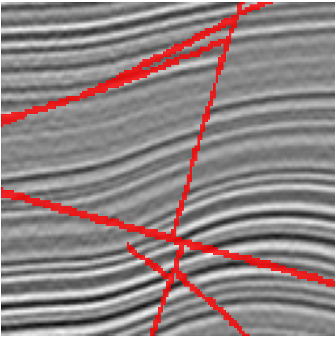
GRvA Synthetic — Fault Overlay Slice Y=64 (crossline)
