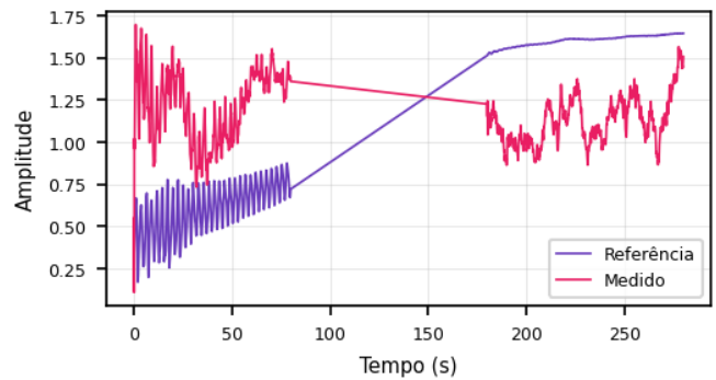
Pitch: Refer. vs. Medido (-25.12%)
