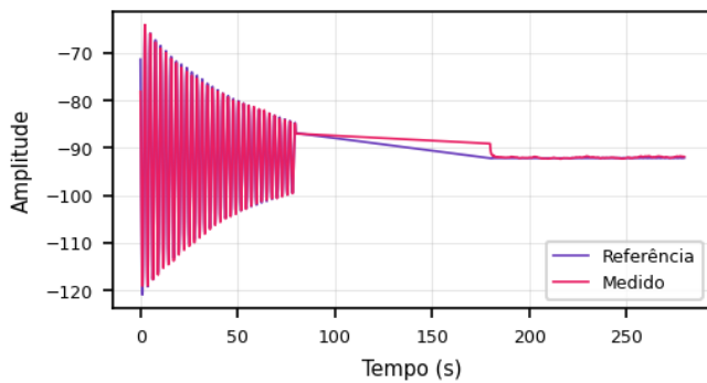
Roll: Refer. vs. Medido (99.70%)
